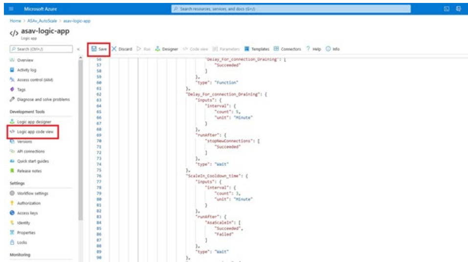
Figure 29: Logic App Code View
