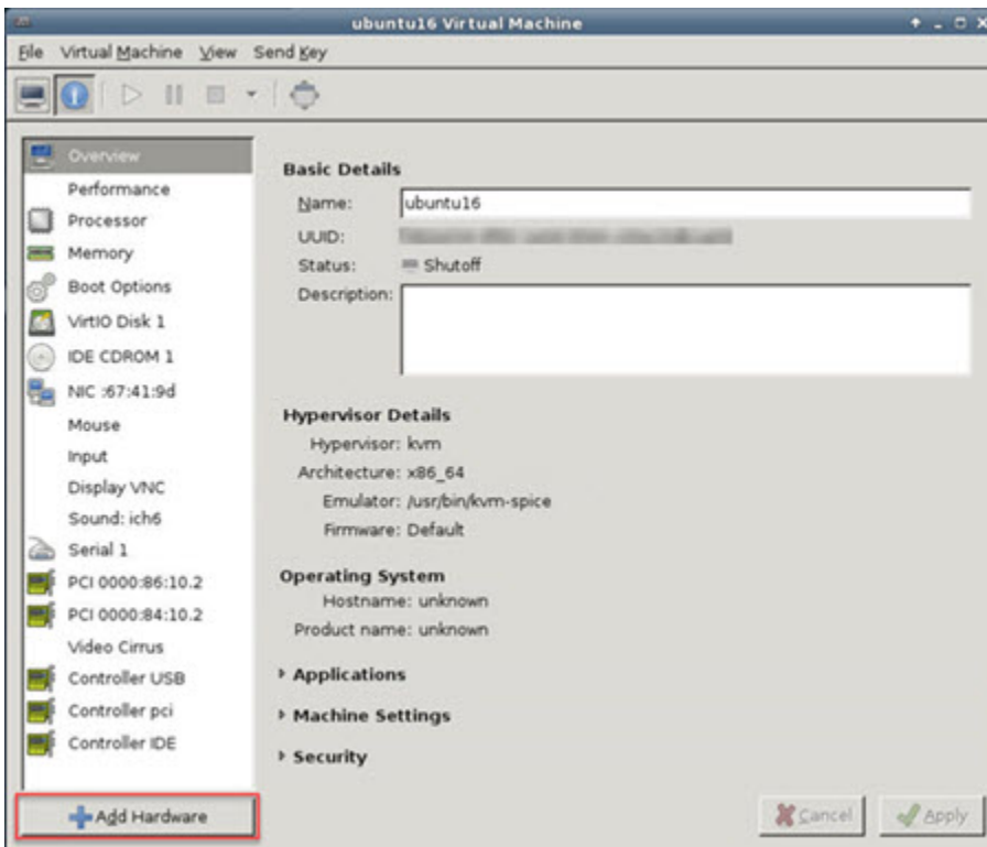
Figure 11: Add Hardware
