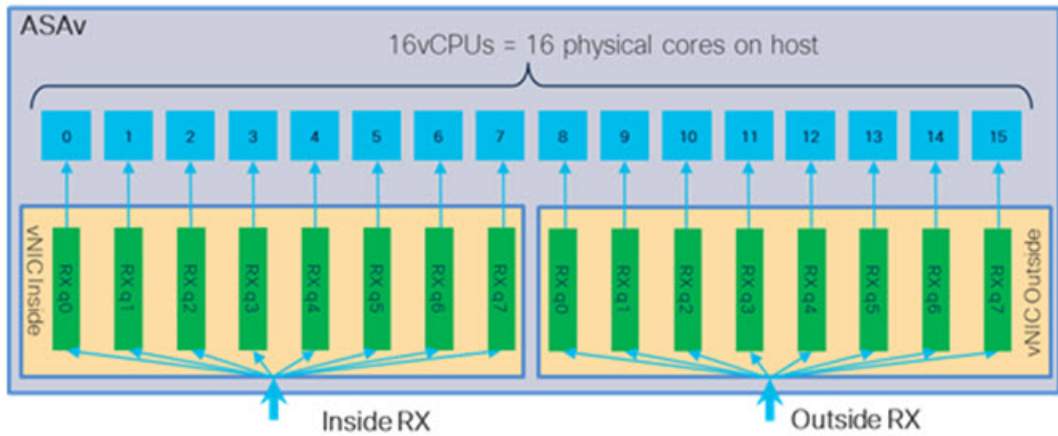
Figure 4: 16-Core ASA RSS RX Queues
