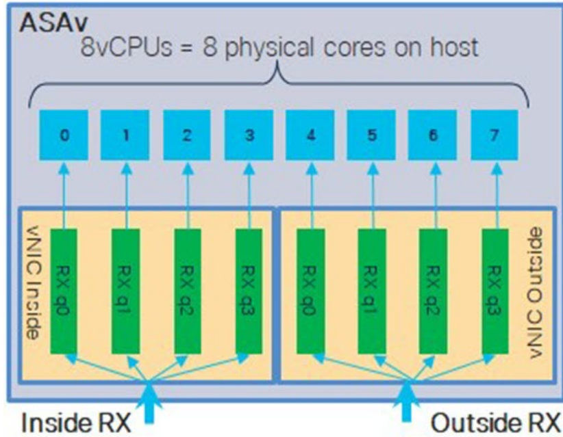
Figure 3: 8-Core ASA RSS RX Queues
