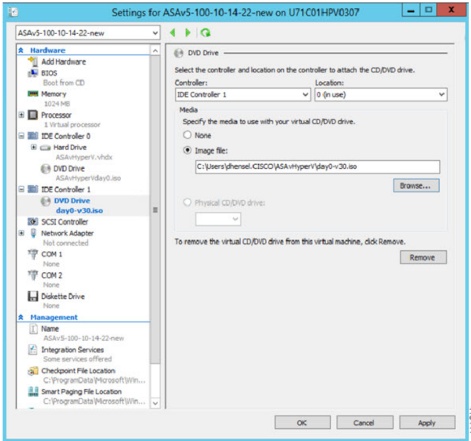
Figure 12: Hyper-V Manager
