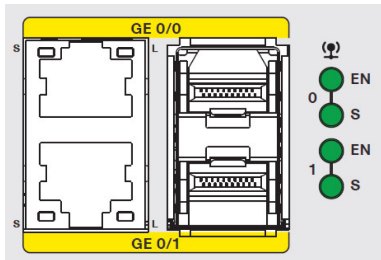
Figure 4: LEDs for Gigabit Ethernet Ports
