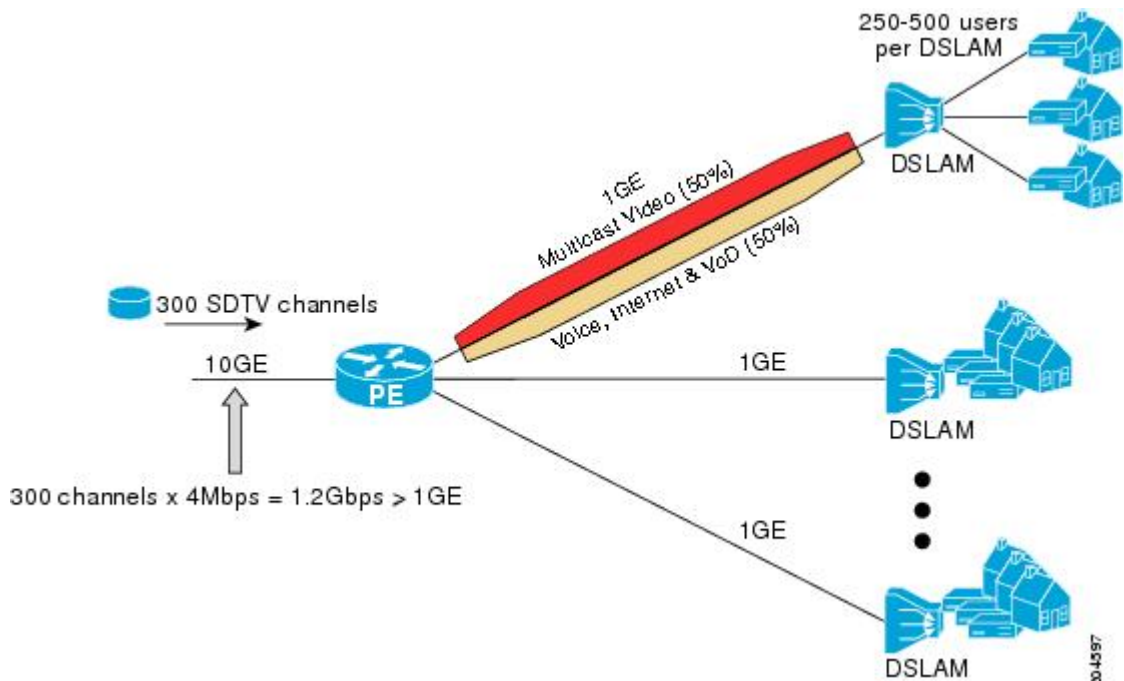
Figure 9: IGMP State Limit Example Topology
