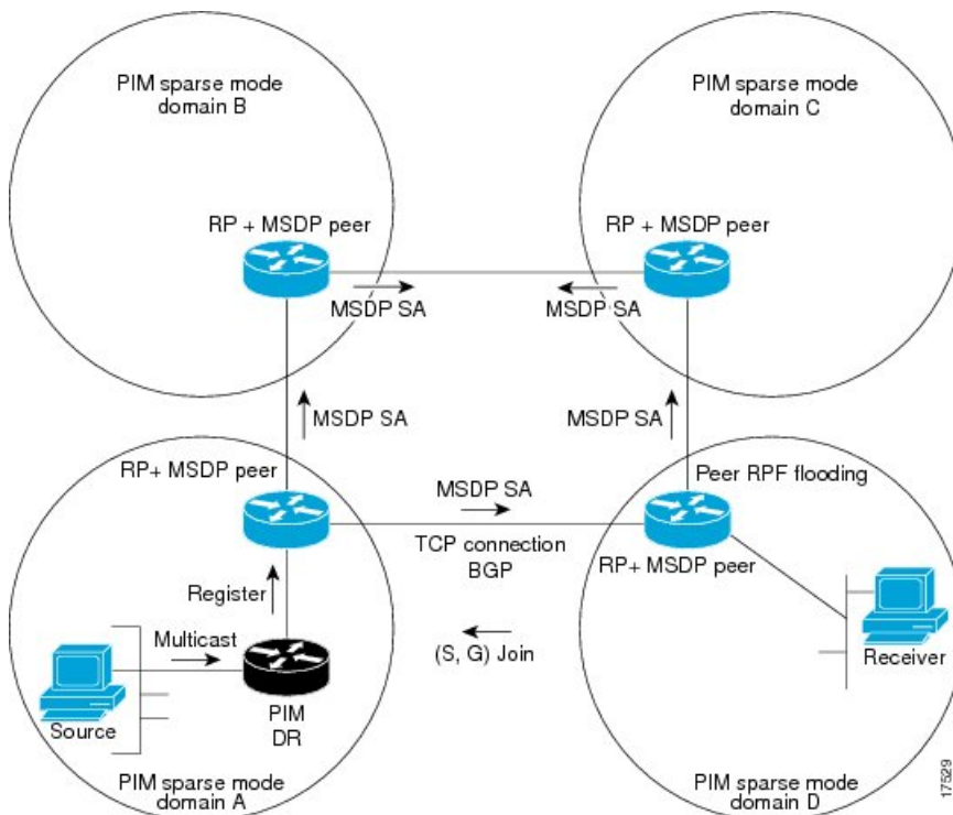
Figure 25: MSDP Running Between RP Peers
