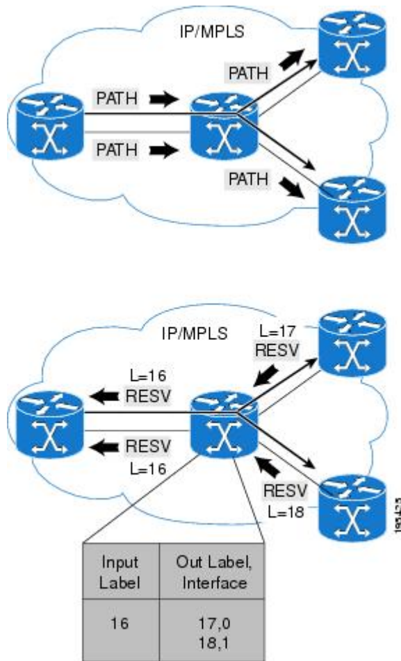
Figure 30: How LSPs Are Signaled
