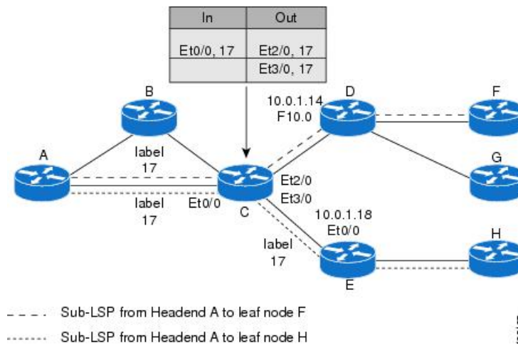
Figure 32: Reusing MPLS Labels in Branch Points
