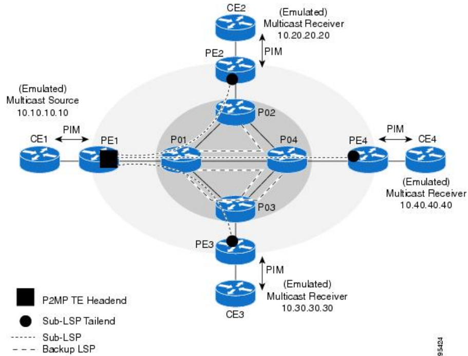
Figure 33: P2MP TE Link Protection Example
