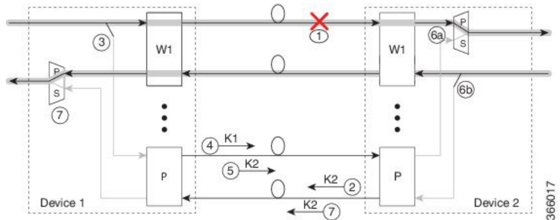
Figure 1: Bidirectional APS 1+1
