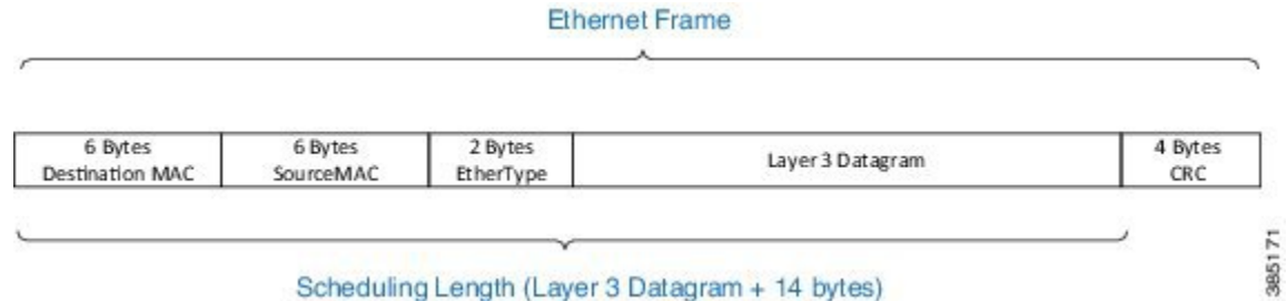
Figure 6: Scheduling Length
