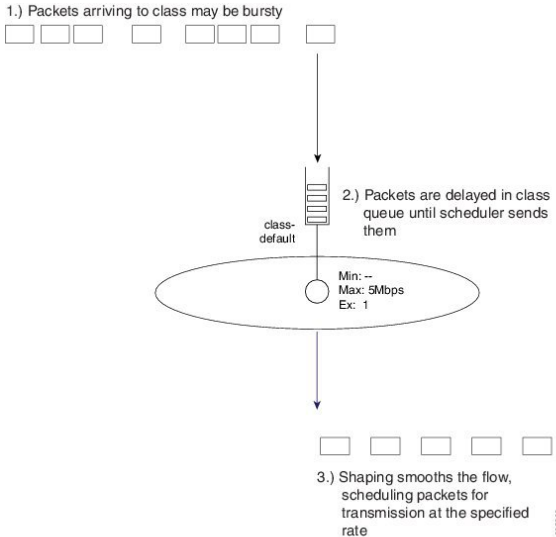
Figure 11: Single-shaped Queue
