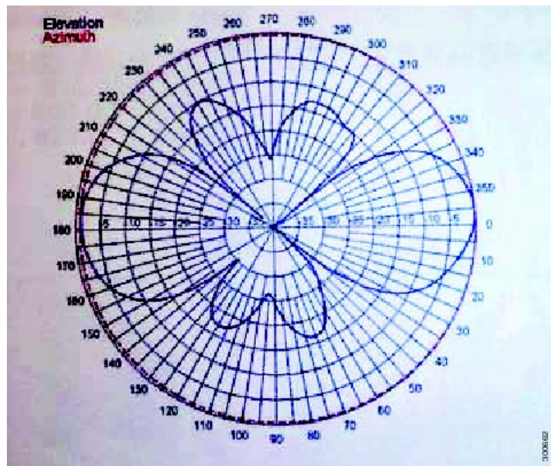
Figure 2: Outdoor Omnidirectional Antenna Radiation Pattern
