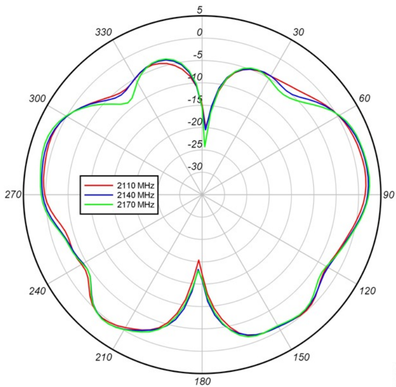
Figure 26: Elevation Plane Patterns ( \Phi = 90 degree Plane Cut) for the 2100 MHz Band
