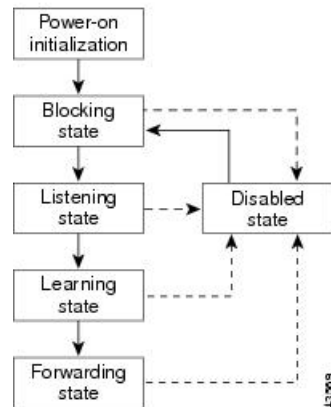
Figure 12: Spanning-Tree Interface States
