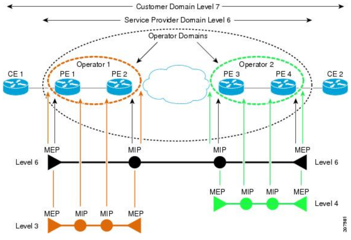
Figure 2: Different CFM Maintenance Domains Across a Network
