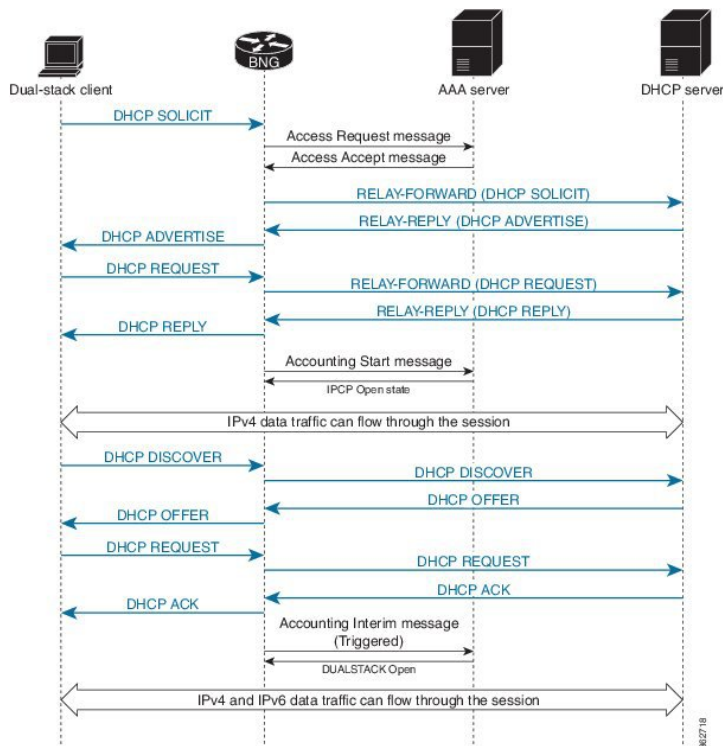
Figure 52: Call Flow of IPoE Dual-Stack - IPv6 Address-Family Starts First
