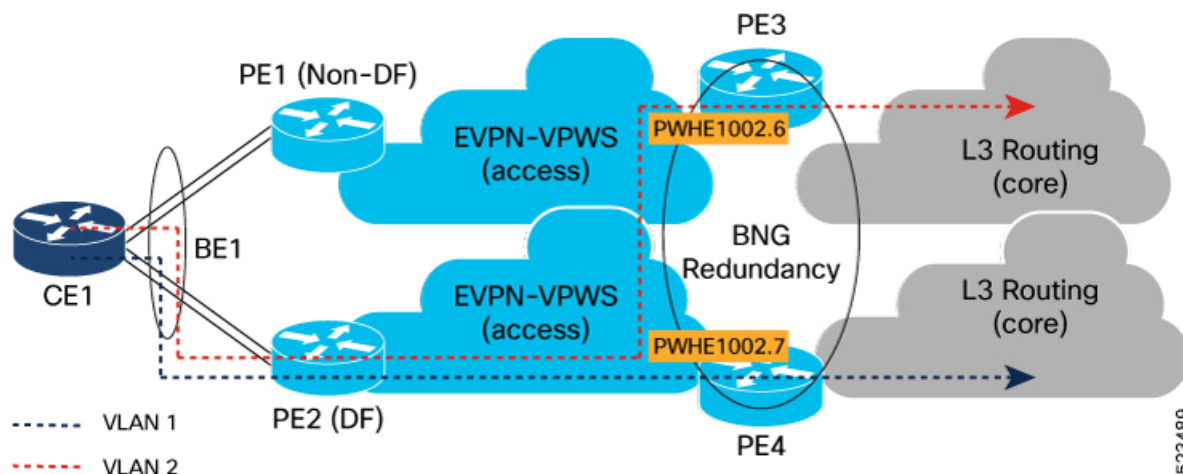
Figure 29: EVPN Geo Redundancy
