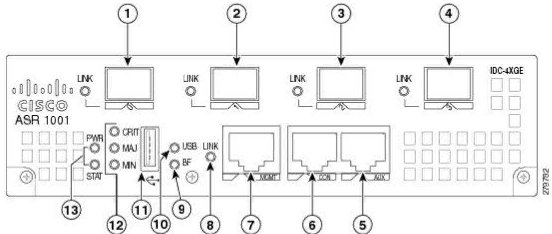
Figure 3: Cisco ASR 1001 Router with IDC-4XGE
