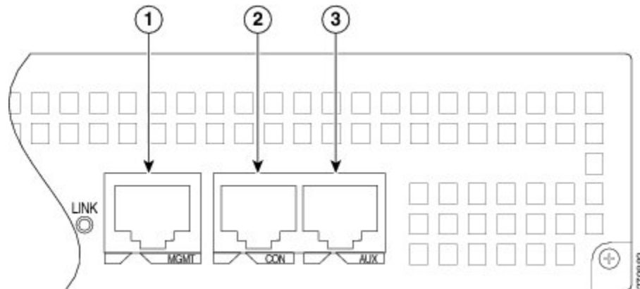
Figure 7: Common Connectors for Cisco ASR 1001 Route Processor
