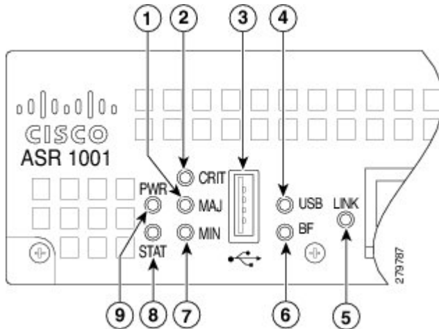
Figure 6: Common LEDs for Cisco ASR 1001 Route Processor
