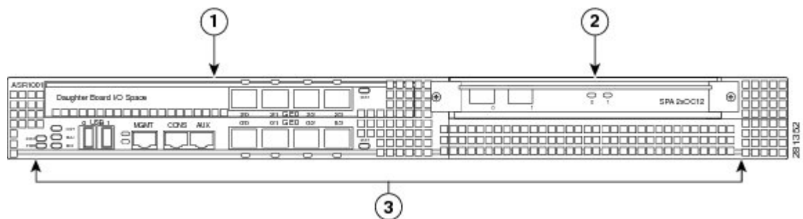
Figure 9: Cisco ASR 1001 Router Slot Numbering
