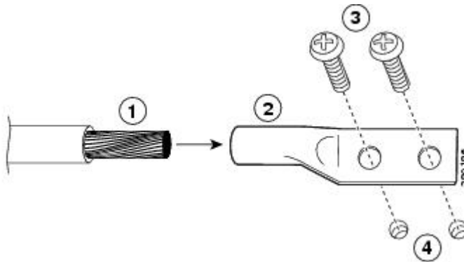
Figure 18: Attaching a Grounding Lug to the Chassis Ground Connector
