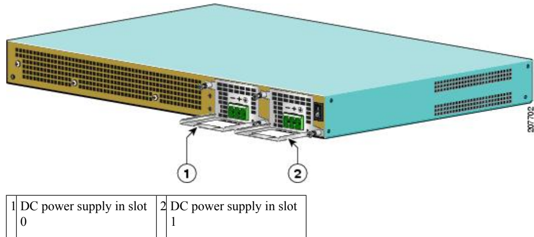
Figure 25: Cisco ASR 1001 Router DC Power Supply Rear View
