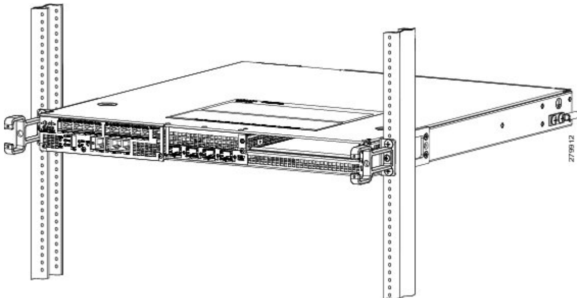
Figure 15: Cisco ASR 1001 Router Installed on a Two-Post Equipment Rack
