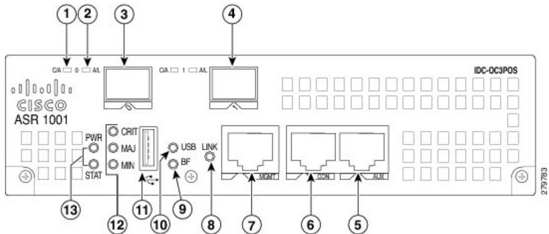
Figure 2: Cisco ASR 1001 Router with IDC-OC3POS
