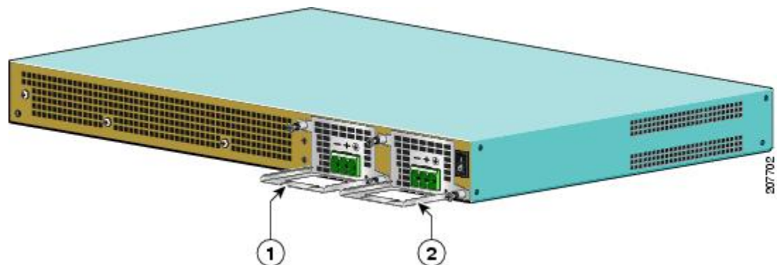
Figure 11: –48 VDC Power Supply for the Cisco ASR 1001 Router
