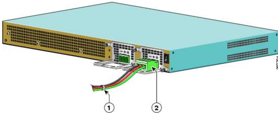
Figure 31: Complete DC Terminal Block Plug Insertion and Secure Tie Wrap
