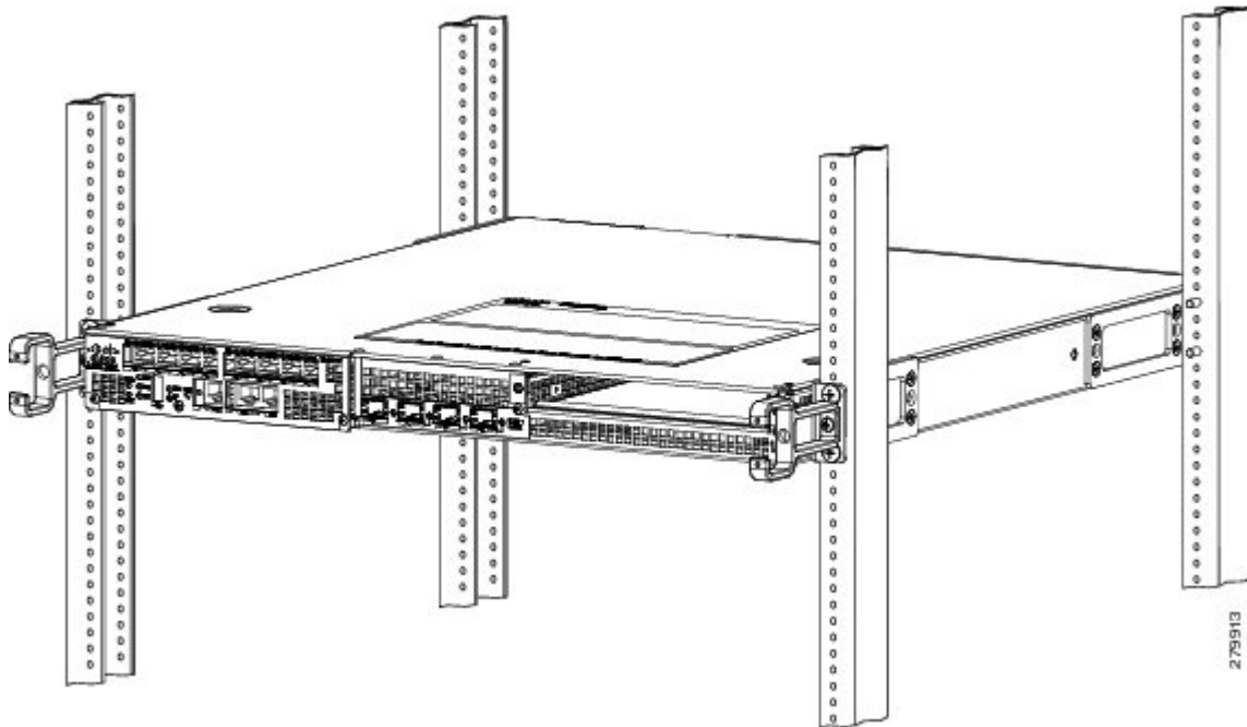
Figure 16: Cisco ASR 1001 Router in a Four Post Rack—Front and Rear Rack-Mounting
