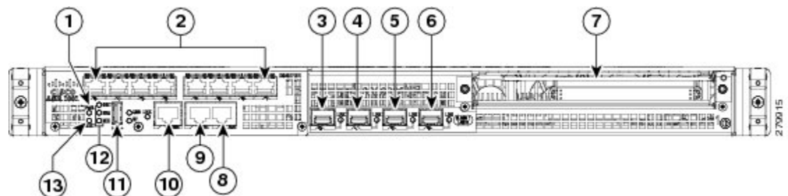
Figure 8: Cisco ASR 1001 Router Front View
