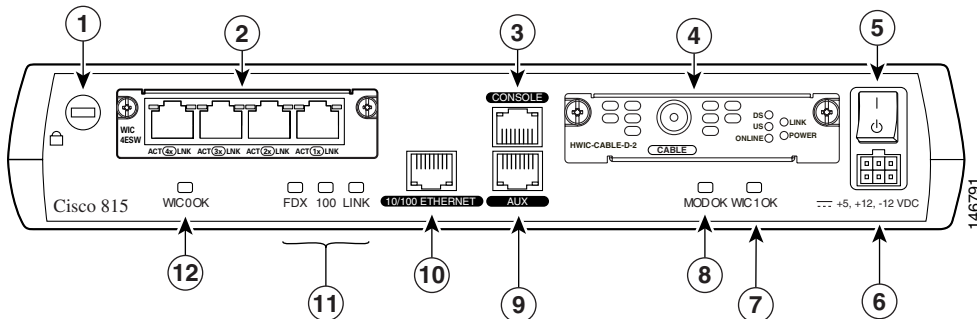
Figure 3 Back Panel
