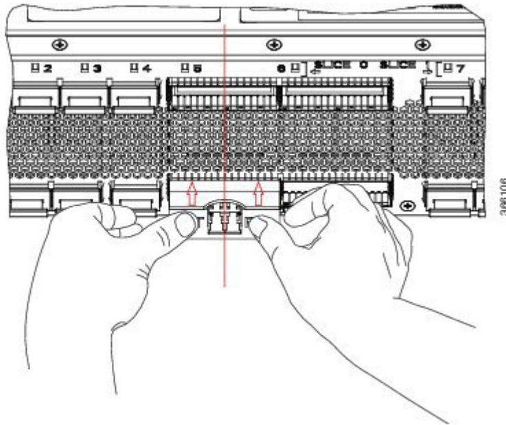
Figure 13: Inserting CFP2-DWDM Pluggable (face-down)
