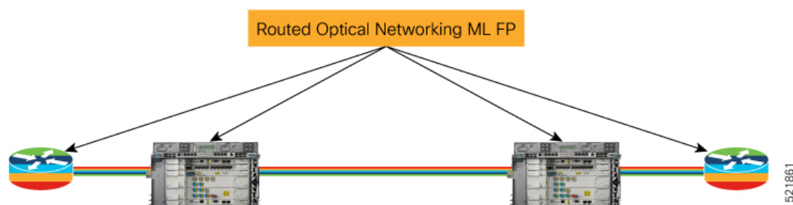
Figure 17: Cisco Routers (with ZR/ZR+ Optics) and NCS 2000 Devices
