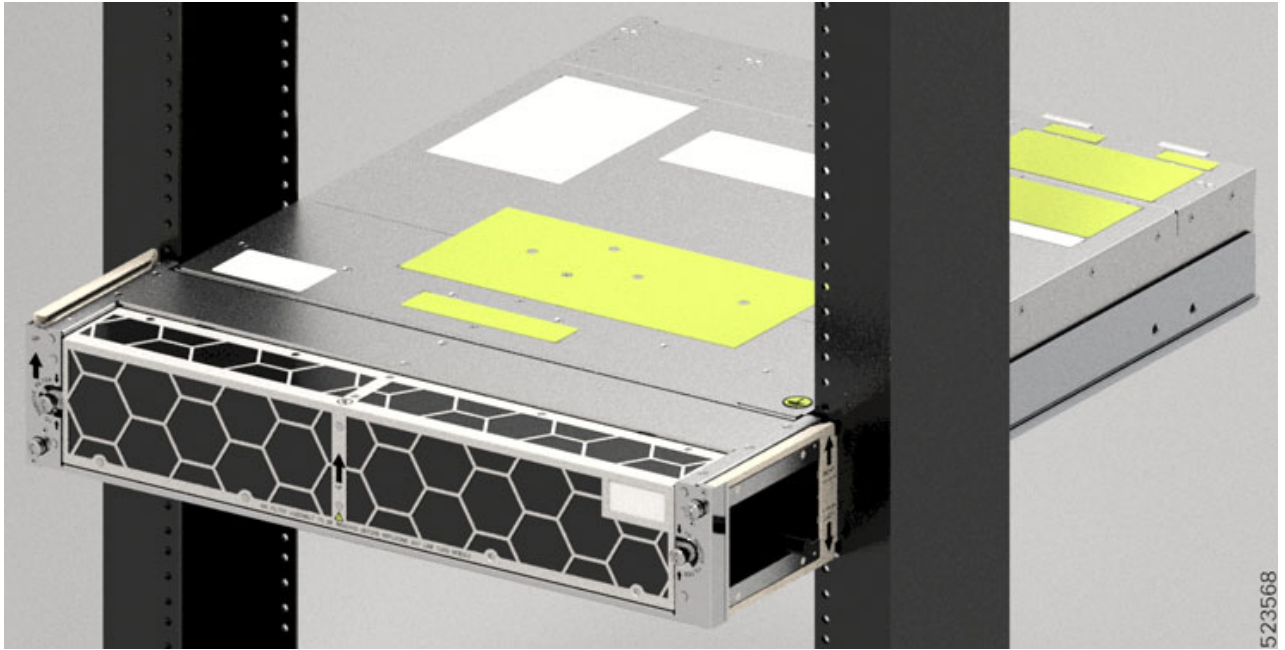
Figure 23: Installed Air Frame
