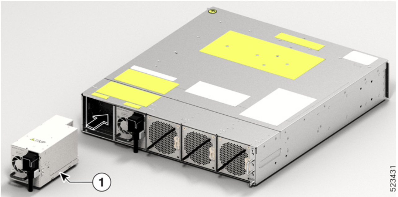
Figure 13: Inserting the PSU
