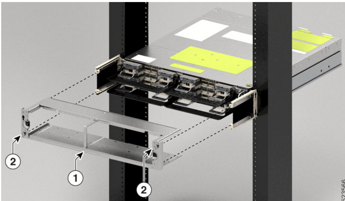
Figure 21: Installing the Air Filter Frame
