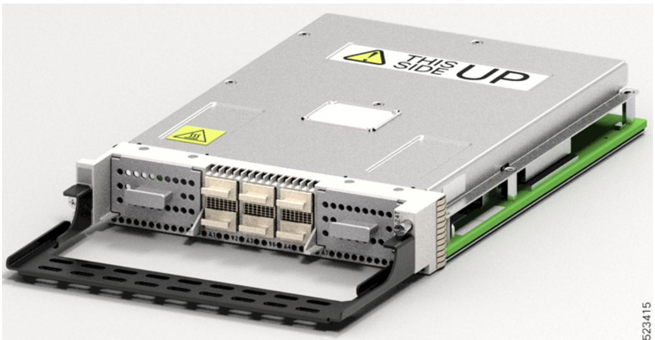
Figure 9: Perspective View of NCS1K14-24T-K9 Line Card
