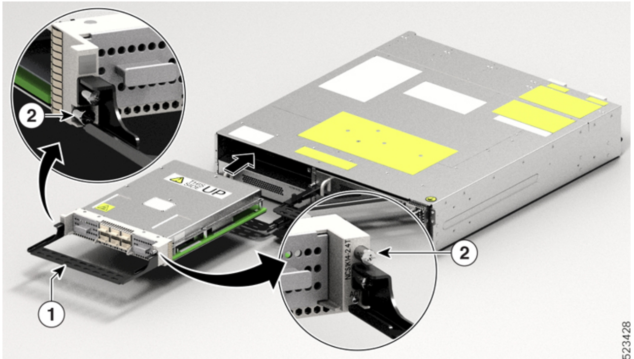
Figure 10: Inserting the NCS1K14-2.4T-K9 Line Card
