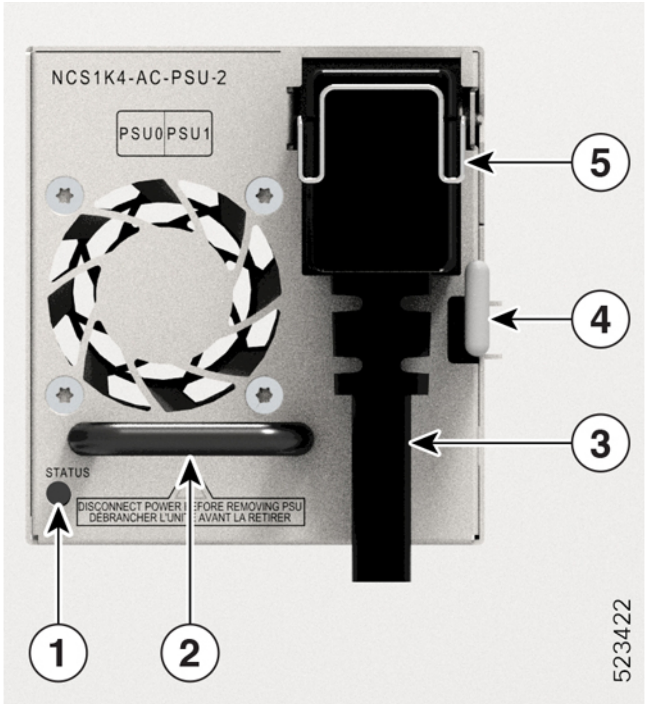
Figure 17: NCS1K4-AC-PSU-2 with 180-Degree Cable Connection
