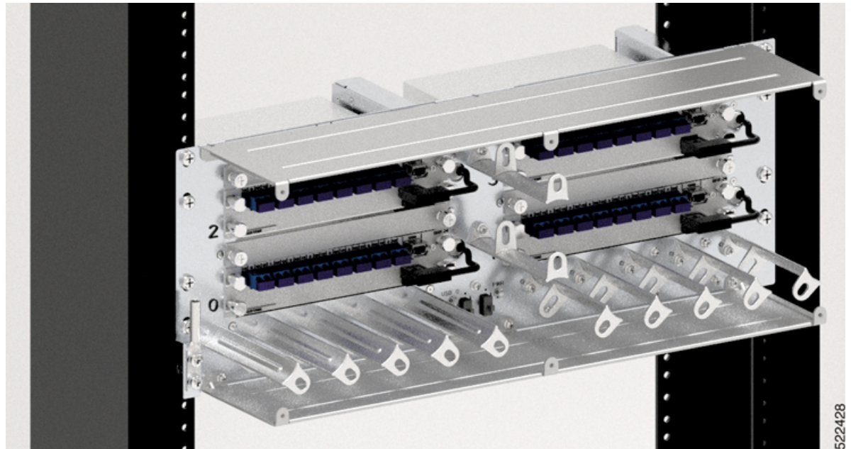
Figure 110: Breakout Panel with Breakout Modules Installed
