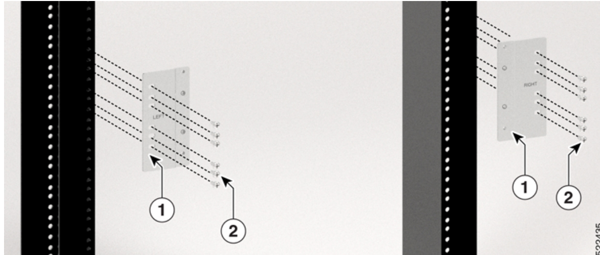
Figure 96: Installing the Adapter Brackets on the 23-inch Rack
