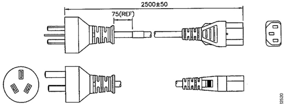
Figure 129: CAB-9K10A-AU (Australia)
