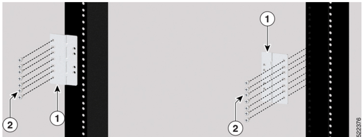
Figure 57: Fixing 23" Adapter
