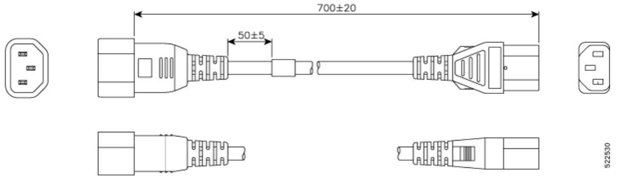
Figure 144: CAB-C13-C14-2M
