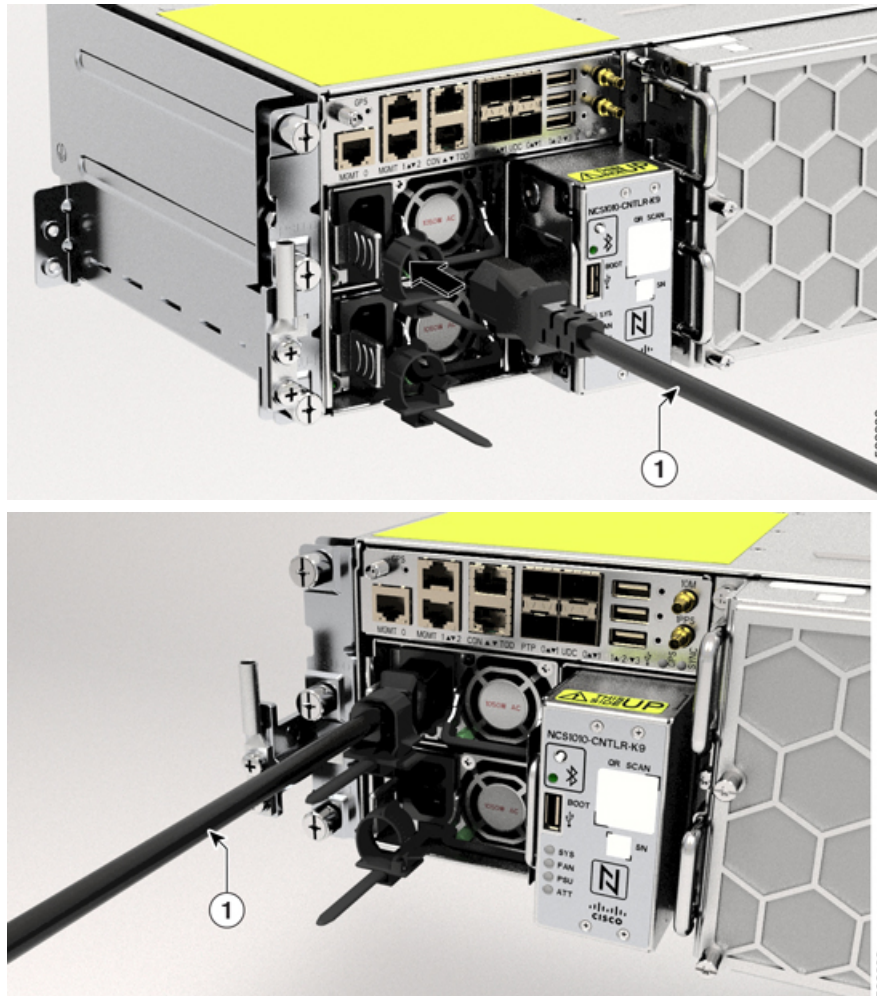
Figure 67: Connecting AC Power Cable
