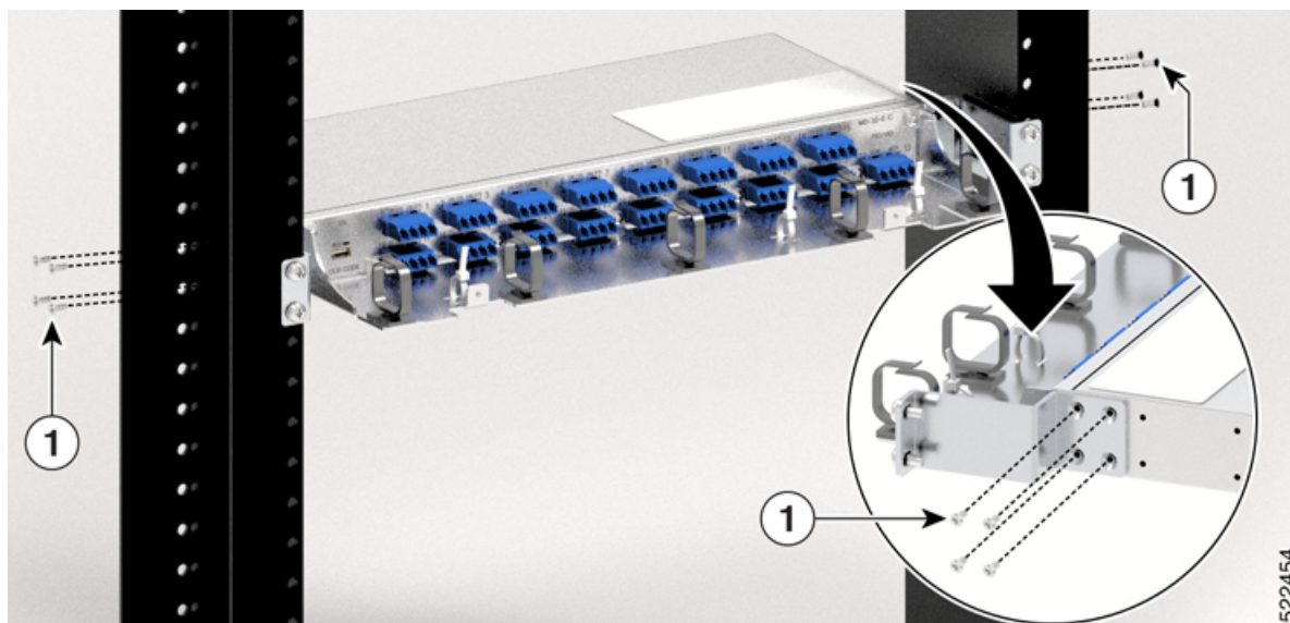
Figure 125: Mounting the Patch Panel on the ETSI Rack
