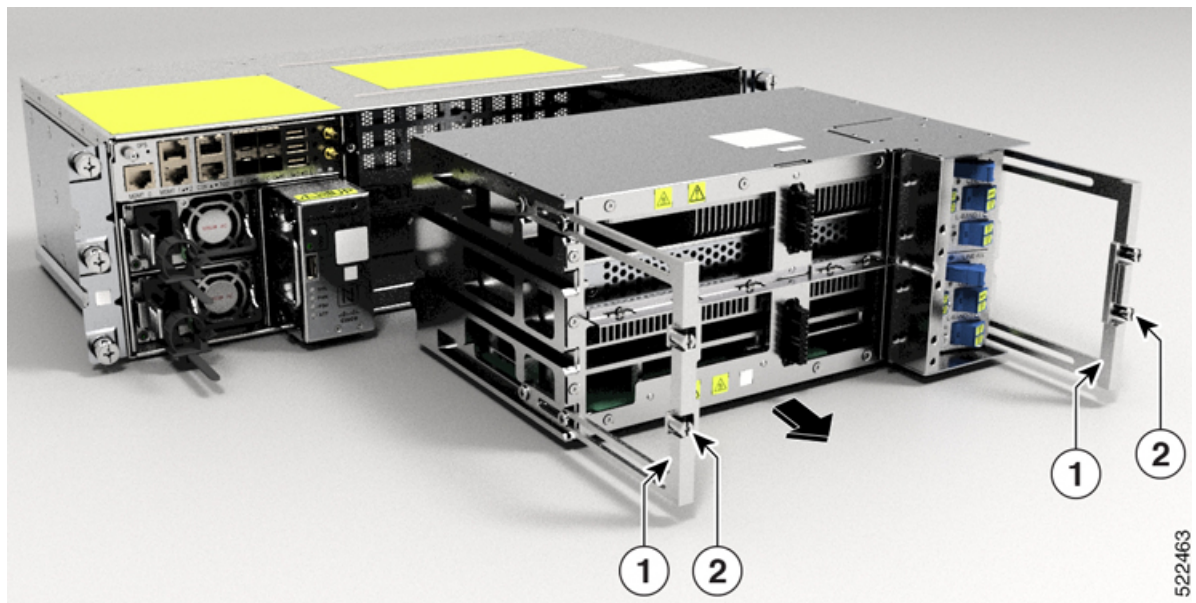
Figure 85: Removing the Line Card
