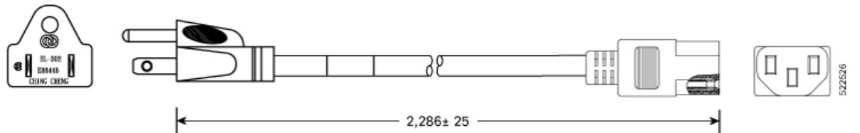
Figure 139: CAB-ACTW (Taiwan)
