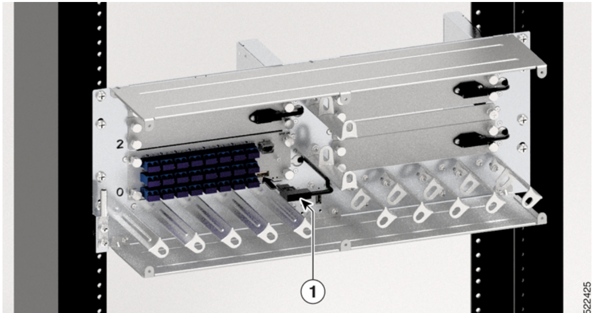
Figure 109: Connecting USB 2.0 Connector for 24-Port Breakout Module
