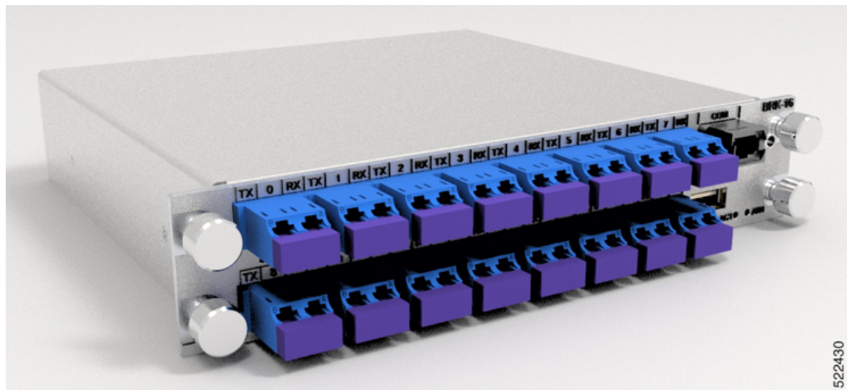
Figure 89: 16-port Breakout Module
