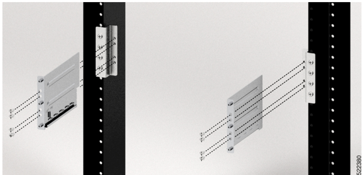
Figure 60: Slide Rail Integration - ETSI Rack
