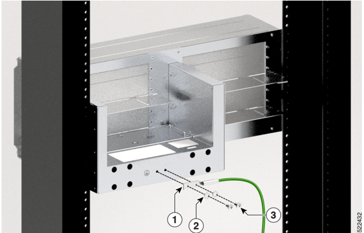
Figure 95: Rear Side Grounding Option
