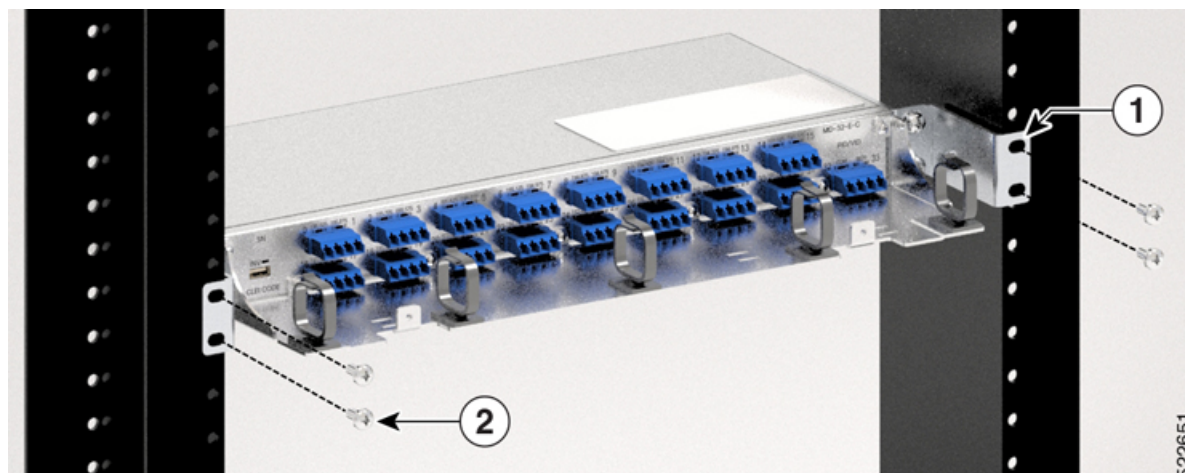
Figure 124: Installing the Mounting Bracket on an ETSI Rack
