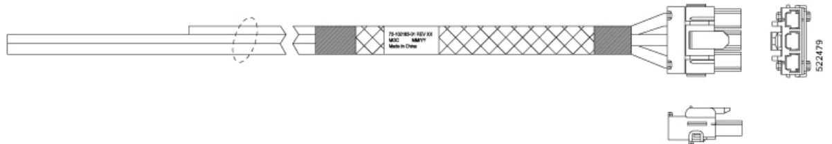
Figure 146: CAB-48DC-40A-8AWG (Worldwide)
