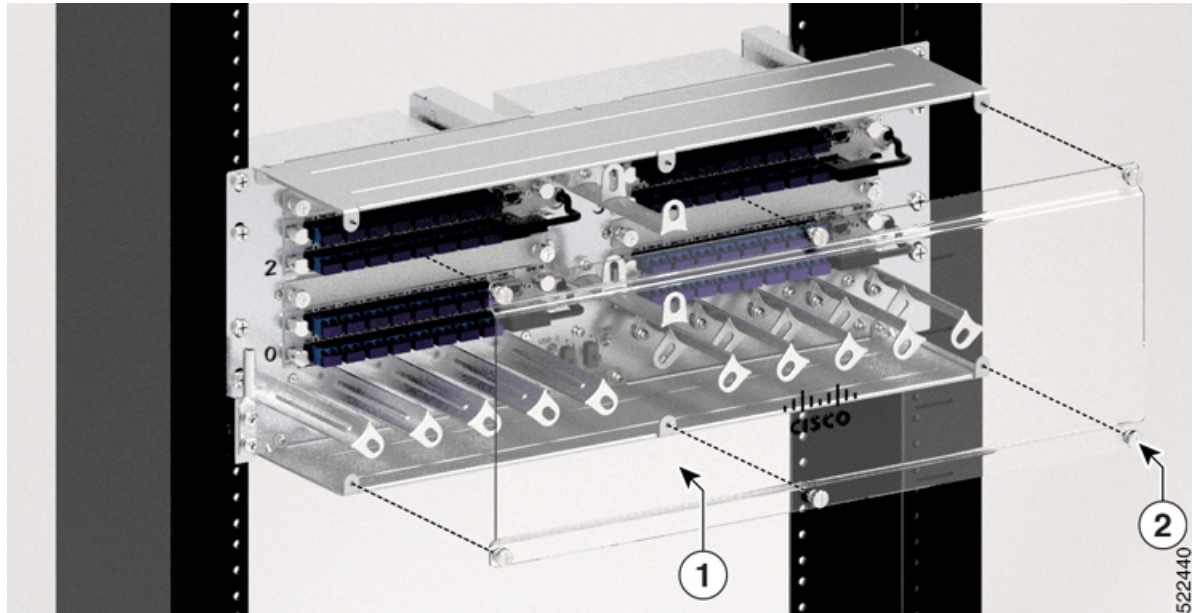
Figure 117: Installing the Plastic Cover on Breakout Panel
