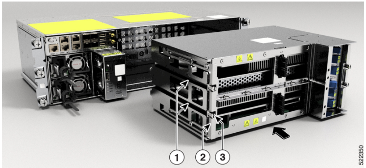
Figure 72: Inserting the Line Card
