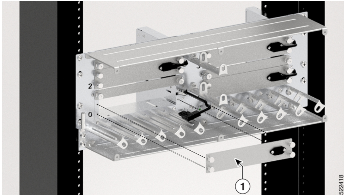
Figure 103: Removing USB Dummy Cover for 8/16-Port Module
