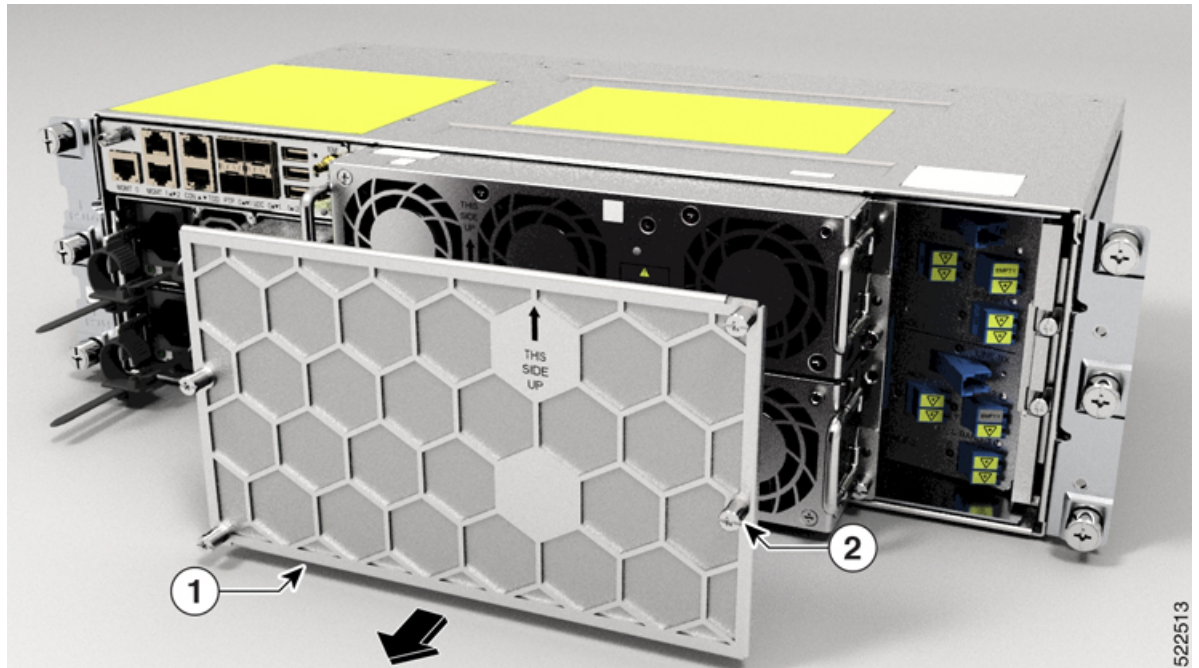
Figure 83: Removing the Fan Filter
