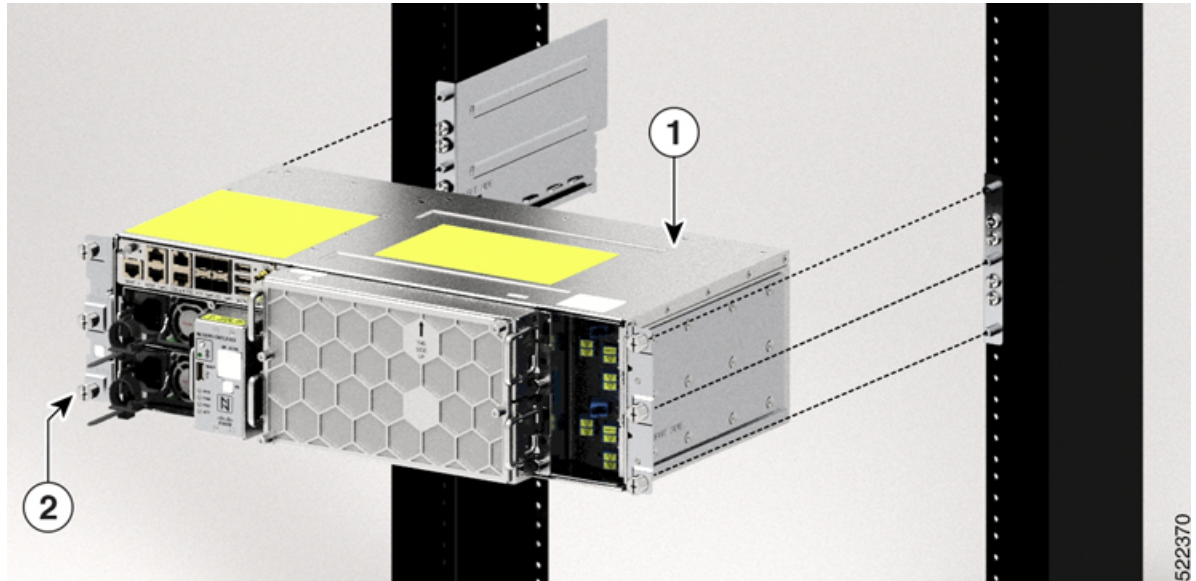
Figure 64: Mounting the Chassis on the Rack
