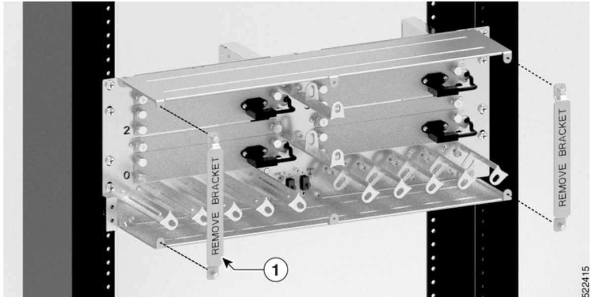
Figure 101: Removing Front Brackets from Breakout Panel
