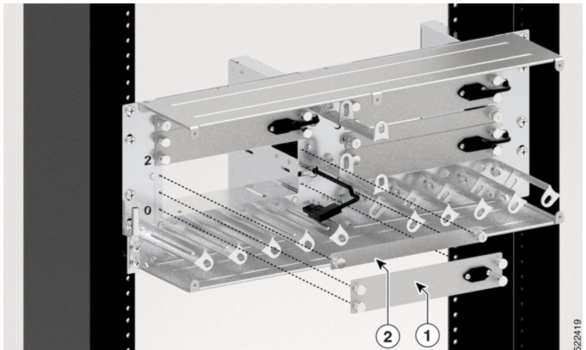
Figure 104: Removing Dummy Cover for 24-Port Module
