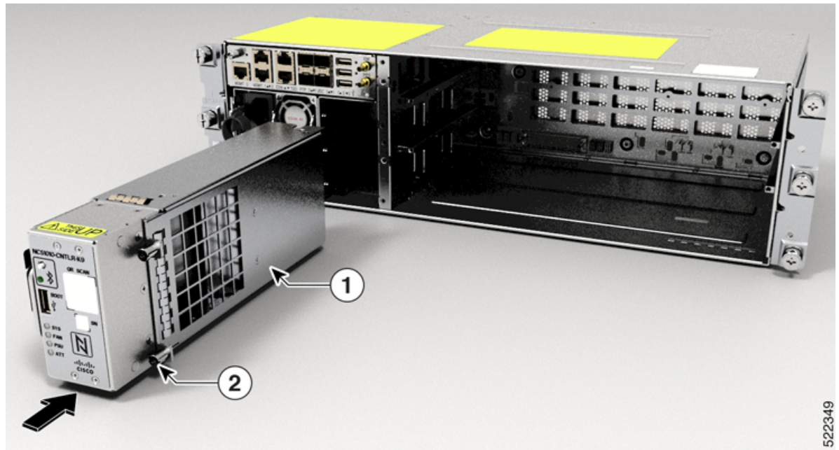
Figure 70: Installing the Controller
