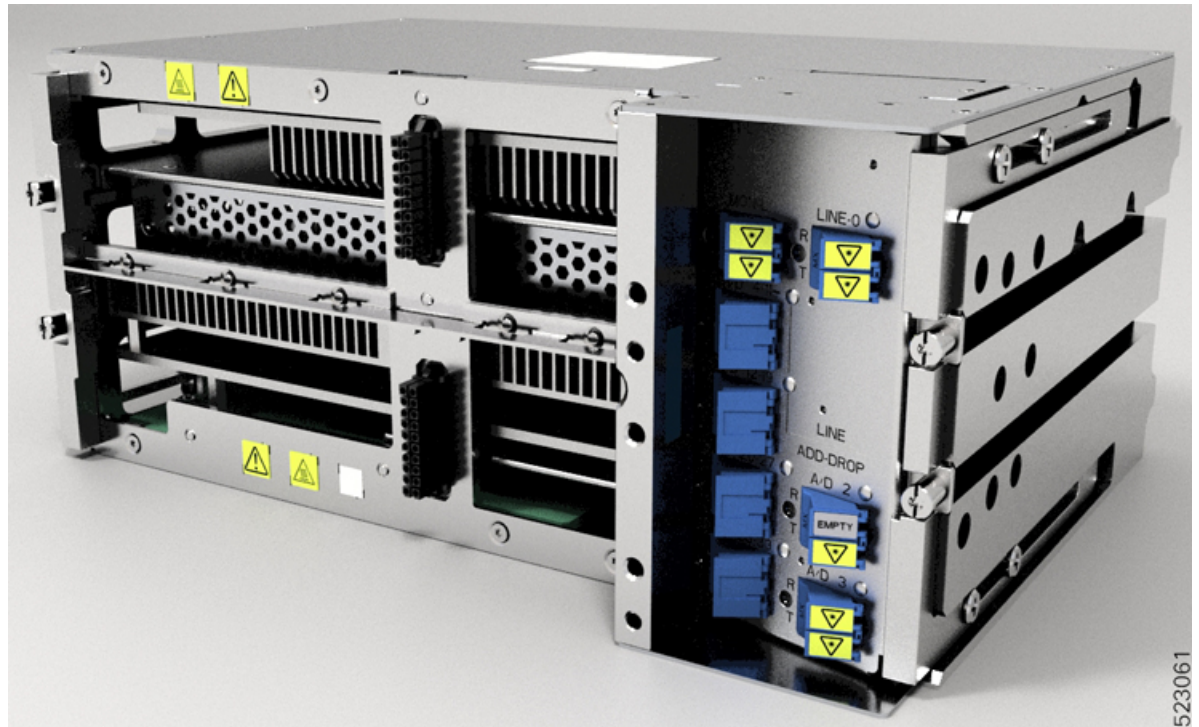
Figure 9: Perspective View of OLT-L Line Card
