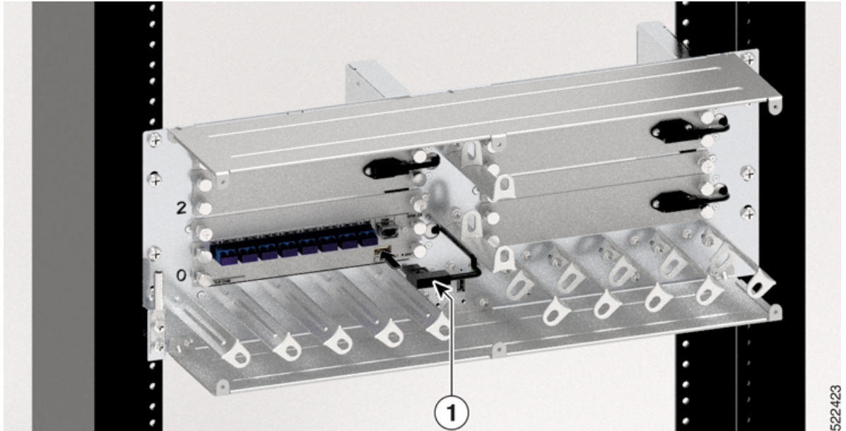
Figure 108: Connecting USB 2.0 Connector for 8-Port Breakout Module
