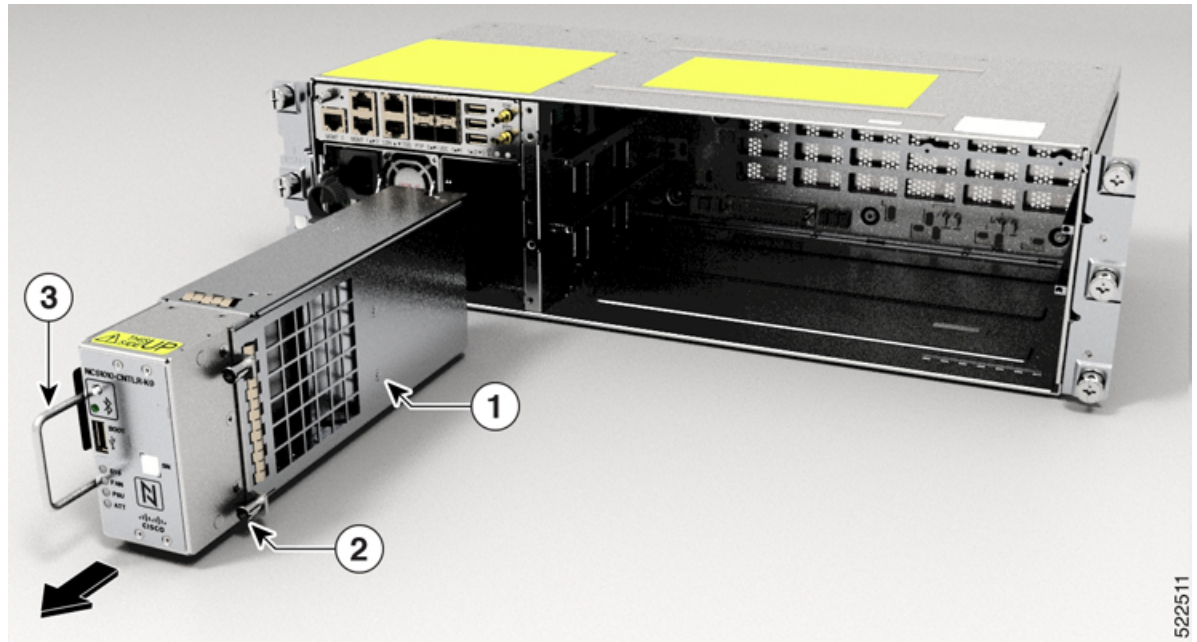
Figure 79: Removing the Controller
