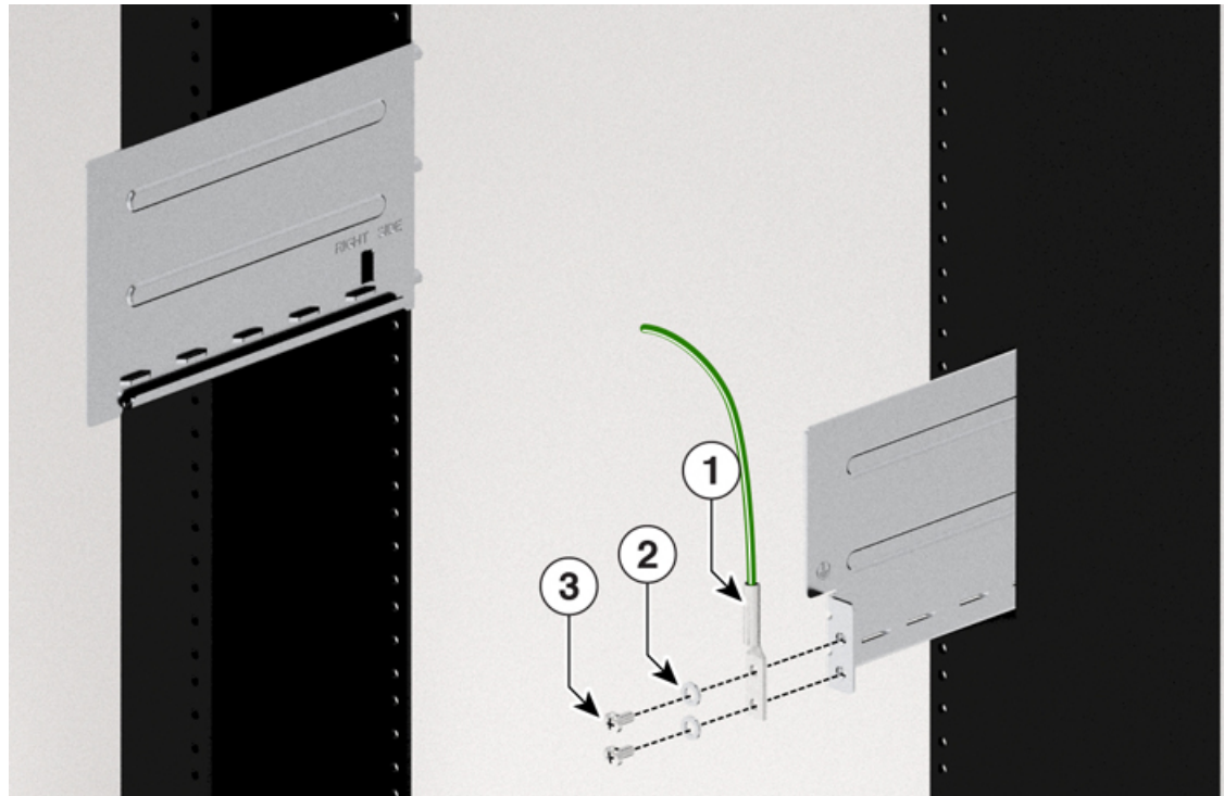
Figure 62: Fixing Ground Lug in the Rear Side of the Slide Rail
