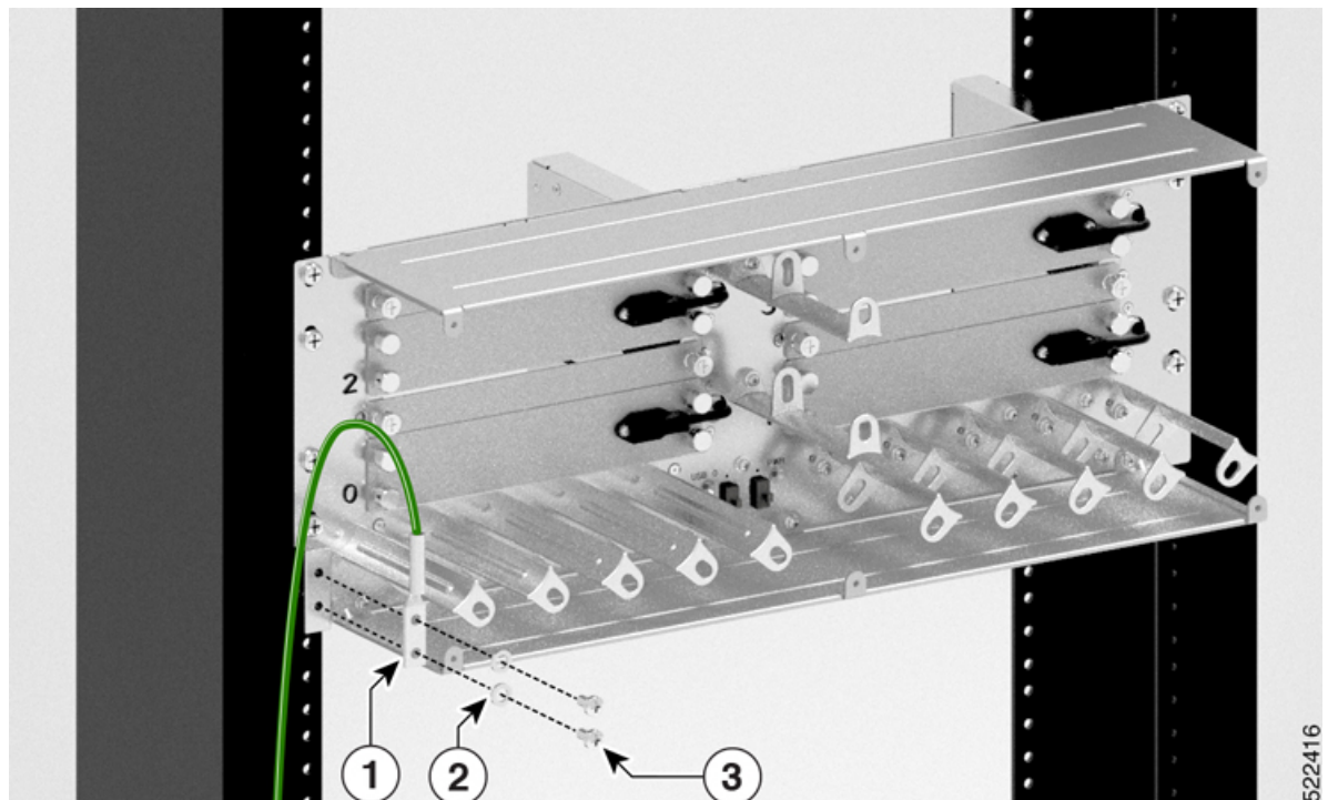
Figure 94: Front Side Grounding Option
