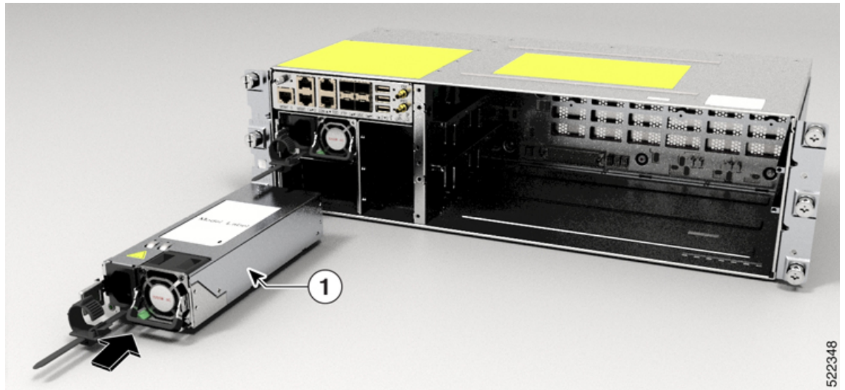
Figure 65: Installing the PSU
