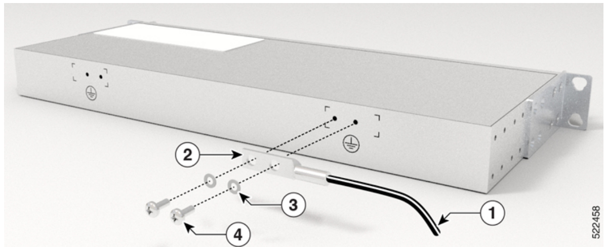
Figure 121: Grounding the Patch Panel
