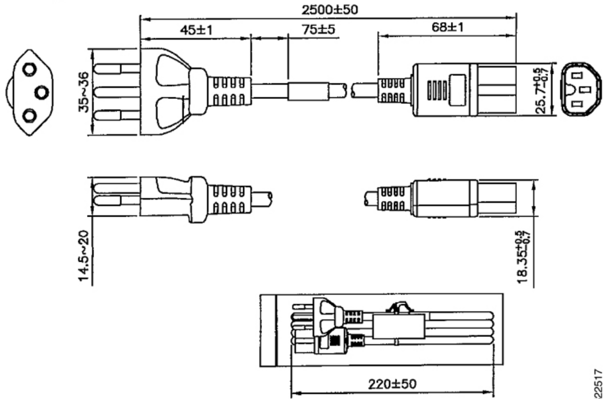
Figure 139: CAB-ACTW (Taiwan)
