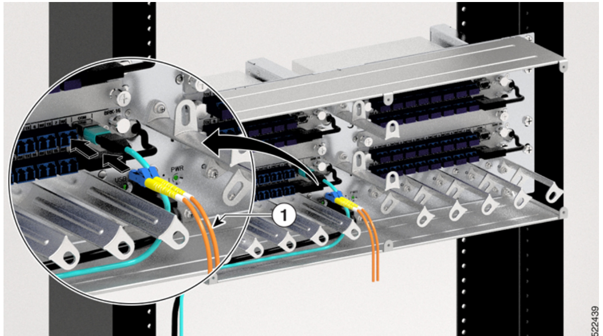
Figure 115: Aligning LC Cable Connector
