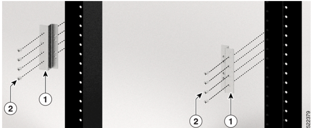
Figure 59: Fixing 19" to ETSI Adapter
