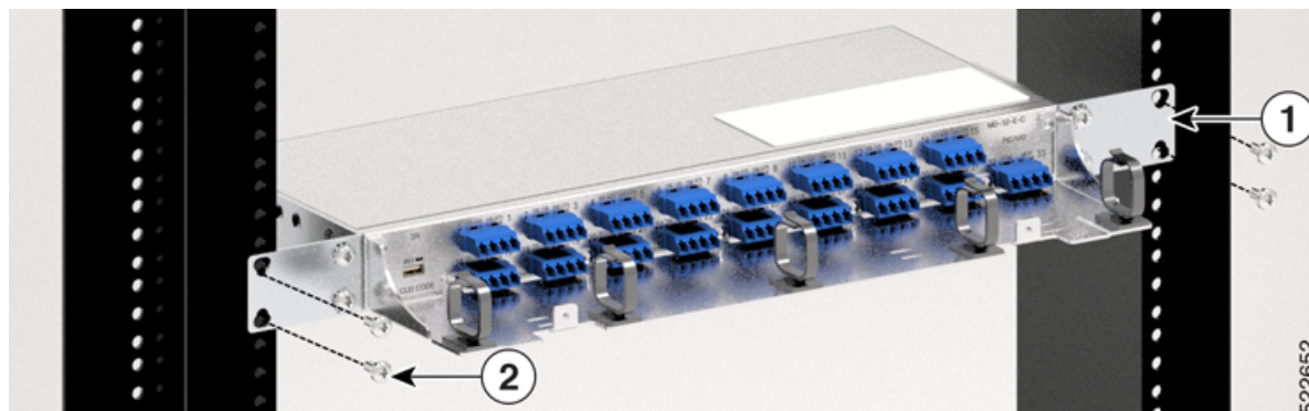
Figure 123: Installing the Mounting Bracket on a 23-inch Rack
