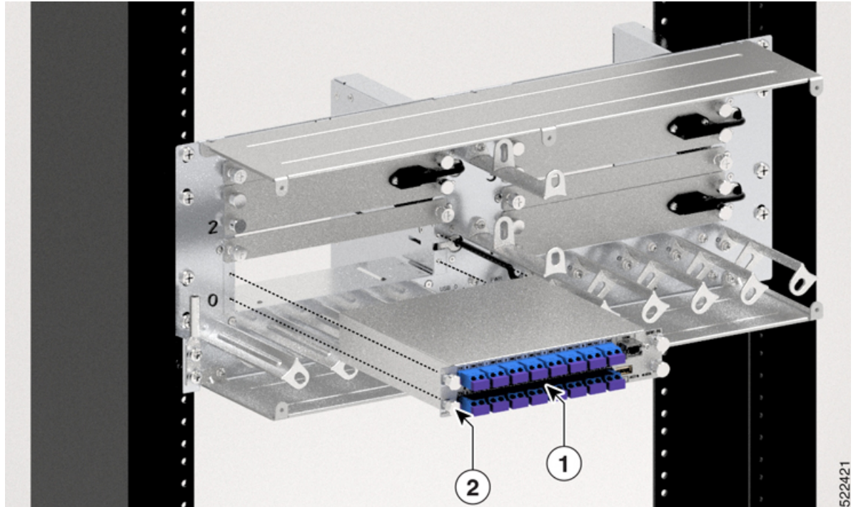
Figure 106: Inserting 16-Port Breakout Module into the Breakout Panel
