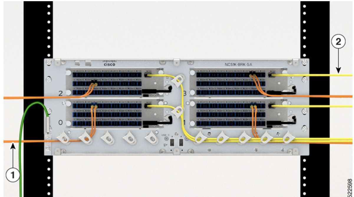
Figure 112: Routing of MPO and LC Cables
