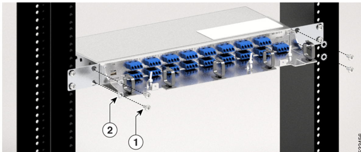
Figure 126: Mounting the Patch Panel on the 23-Inch Rack
