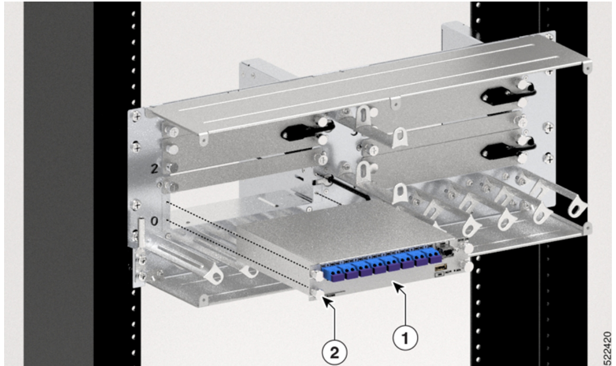
Figure 105: Inserting 8-Port Breakout Module into the Breakout Panel
