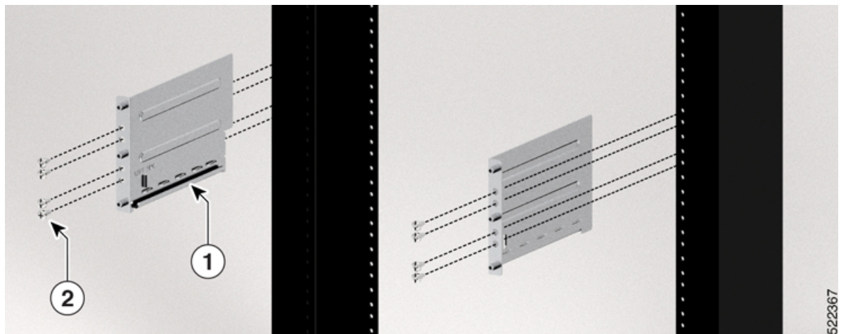
Figure 56: Slide Rail Integration - EIA Rack
