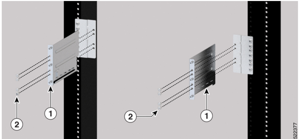
Figure 58: Slide Rail Integration
