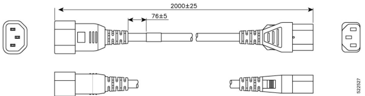
Figure 145: NCS1010-DC-CBL-ET= (Europe)
