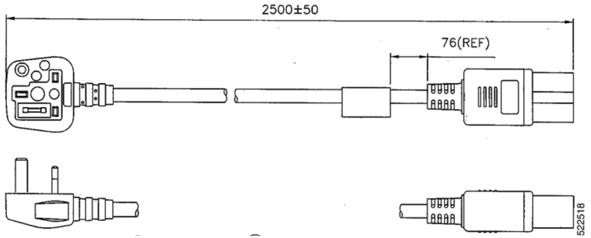
Figure 141: CAB-AC-L620-C13 (North America)
