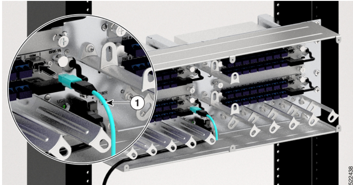
Figure 114: Aligning MPO Fiber Cable Connector
