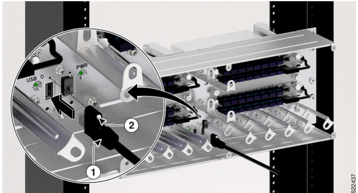
Figure 116: USB 3.0 Cable Connection
