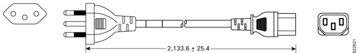
Figure 130: CAB-250V-10A-BR (Brazil)
