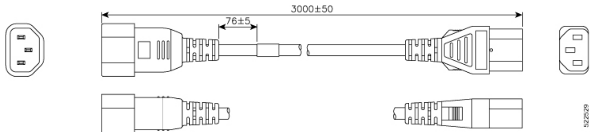
Figure 142: CAB-C13-C14-AC (Europe and North America)
