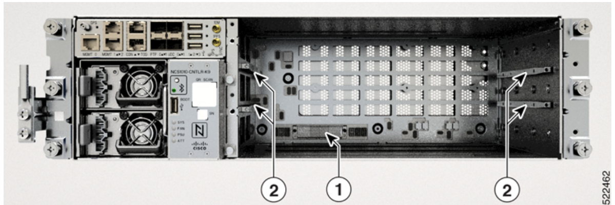
Figure 71: Cisco NCS 1010 Chassis
