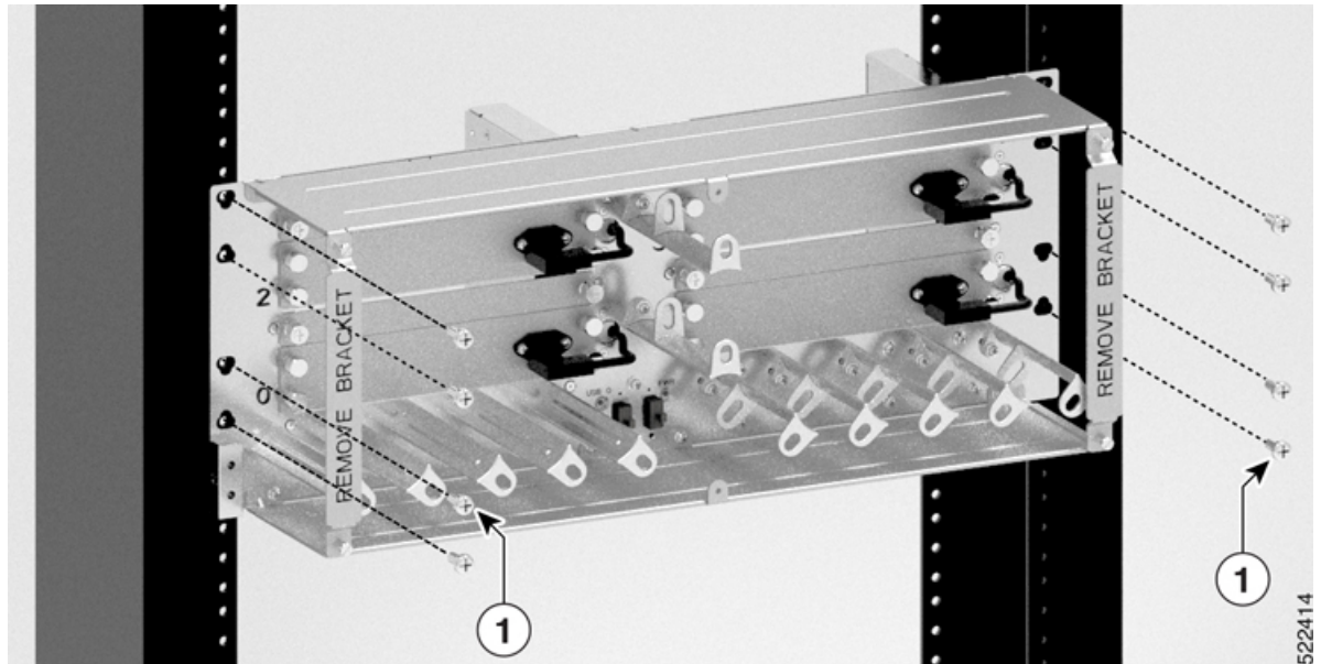
Figure 98: Installing the Breakout Panel on a 19-inch Rack
