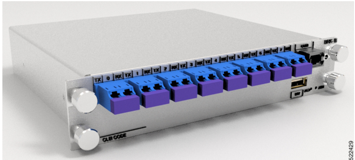
Figure 88: 8-port Breakout Module
