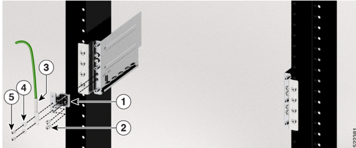
Figure 61: Fixing Ground Lug on the Ground Adapter - ETSI Rack
