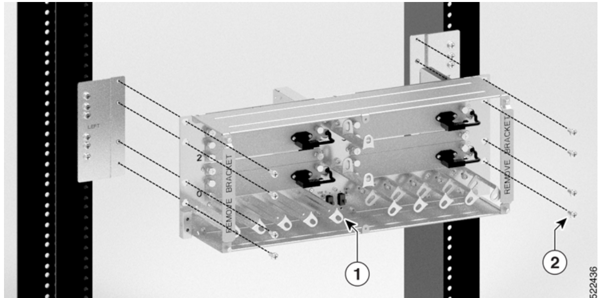
Figure 100: Installing Breakout Panel on a 23-inch Rack
