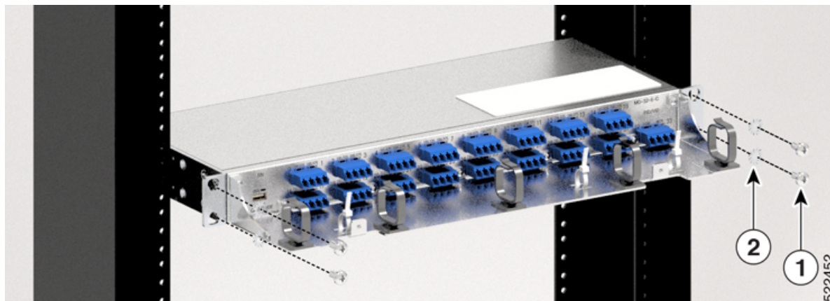
Figure 122: Installing the Adapter Bracket on a 19-inch Rack
