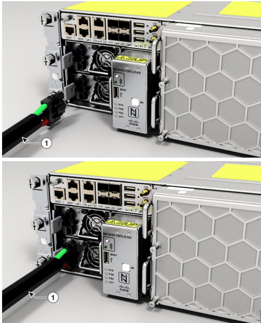
Figure 69: Connecting DC Power
