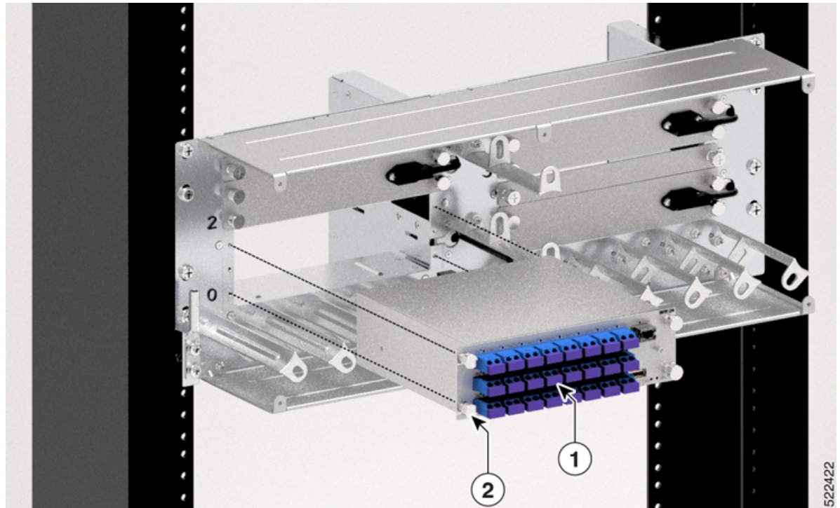
Figure 107: Inserting 24-Port Breakout Module into the Breakout Panel
