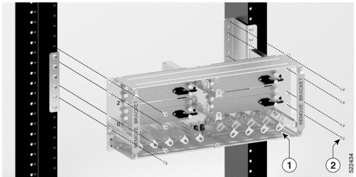
Figure 99: Installing Breakout Panel on an ETSI Rack
