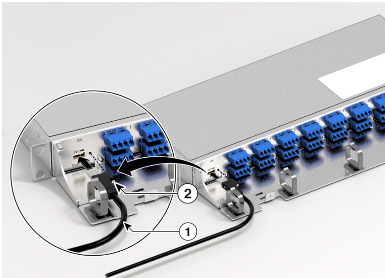
Figure 127: Connecting USB Cable
