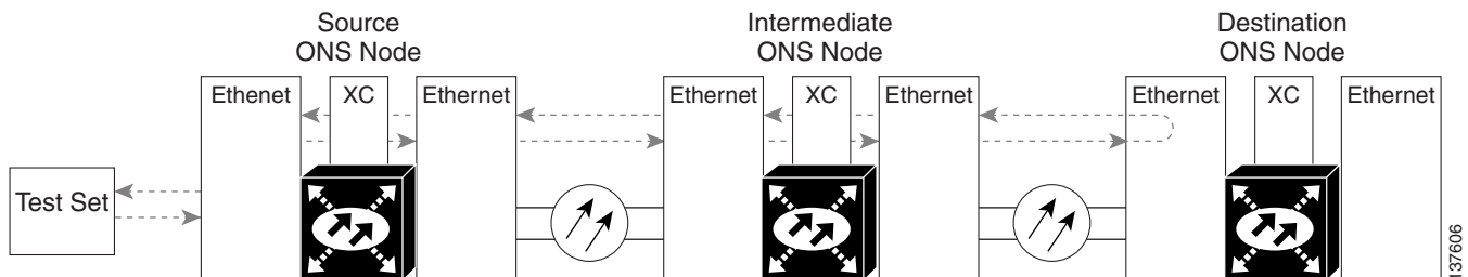
Figure 1-16 Facility Loopback on a Destination-Node Ethernet Port
