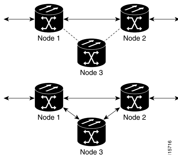
Figure 12-17 Unprotected Point-to-Point ADM to Path Protection Conversion
