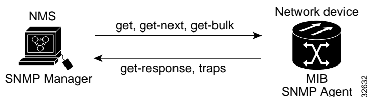
Figure 23-2 SNMP Network
