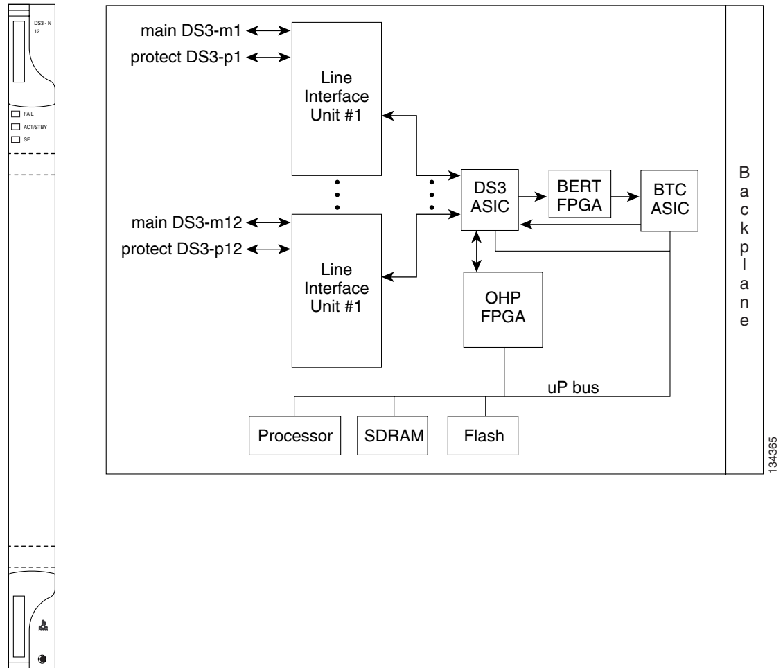
Figure 3-6 DS3i-N-12 Faceplate and Block Diagram
