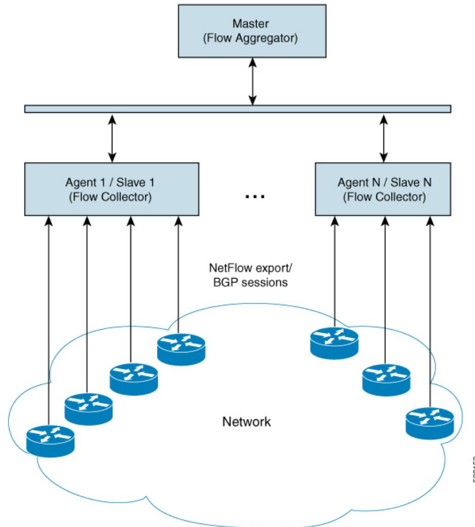
Figure 1: DNF Architecture
