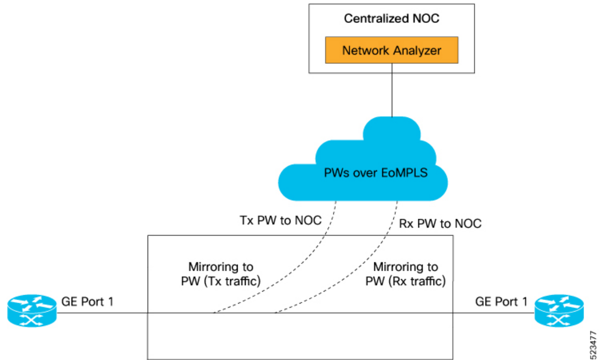
Figure 3: Mirroring Topology
