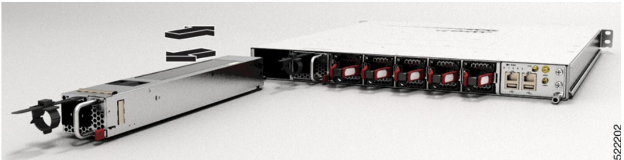
Figure 10: NCS-57C1 - Install AC Power Supply Module
