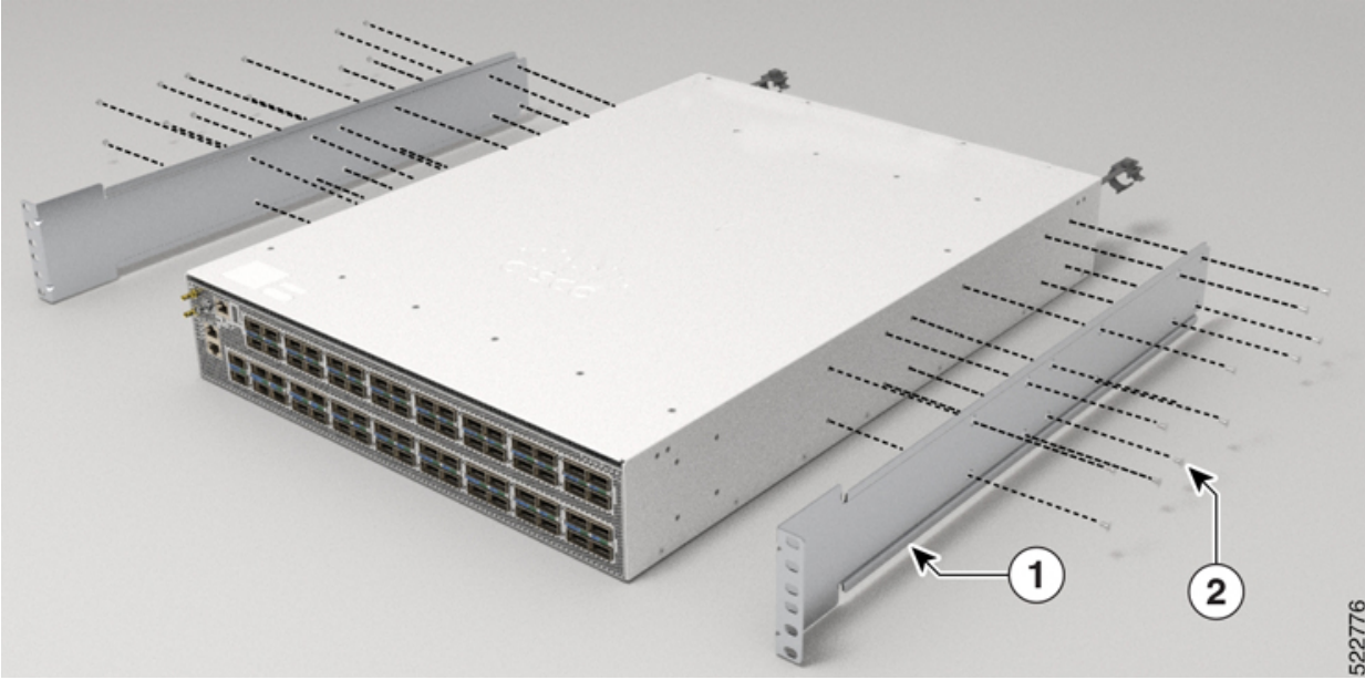
Figure 15: Mount Slider Brackets
