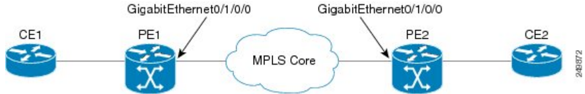
Figure 6: BGP-based VPLS Autodiscovery with BGP signaling
