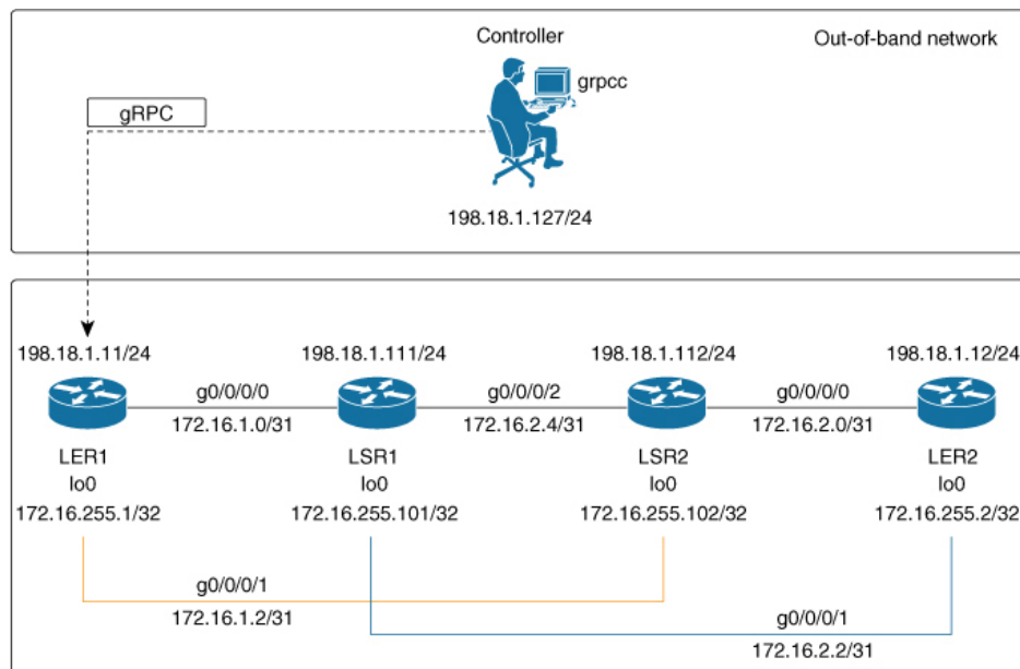
Figure 5: Network Topology for gRPC session
