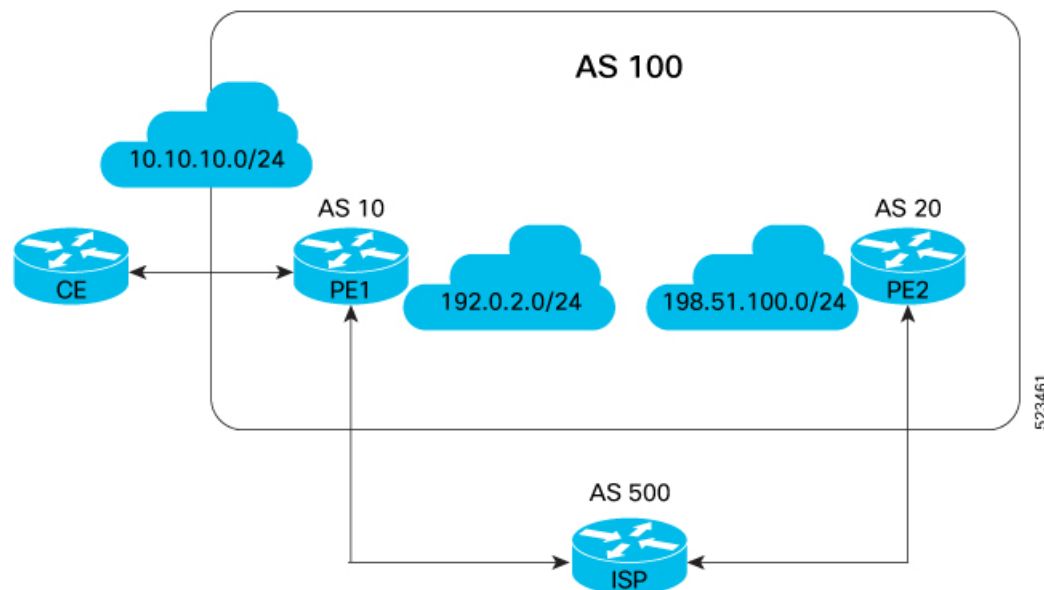
Figure 2: Peering Between BGP Routers Within the Same Confederation
