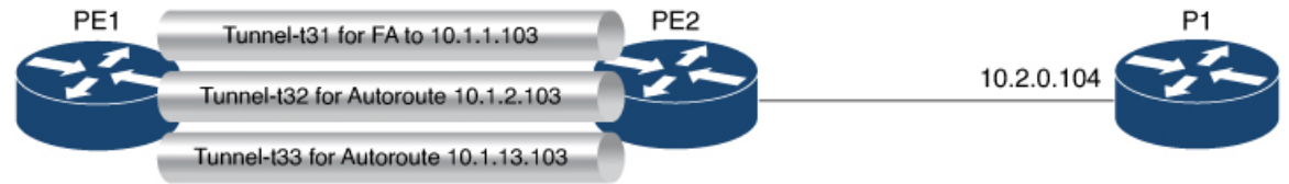
Figure 15: Topology
