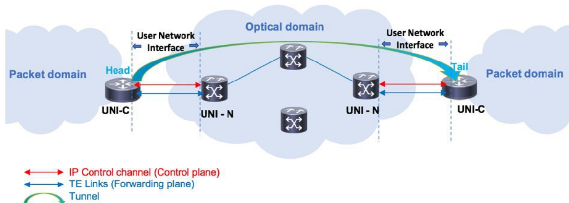
Figure 23: GMPLS UNI
