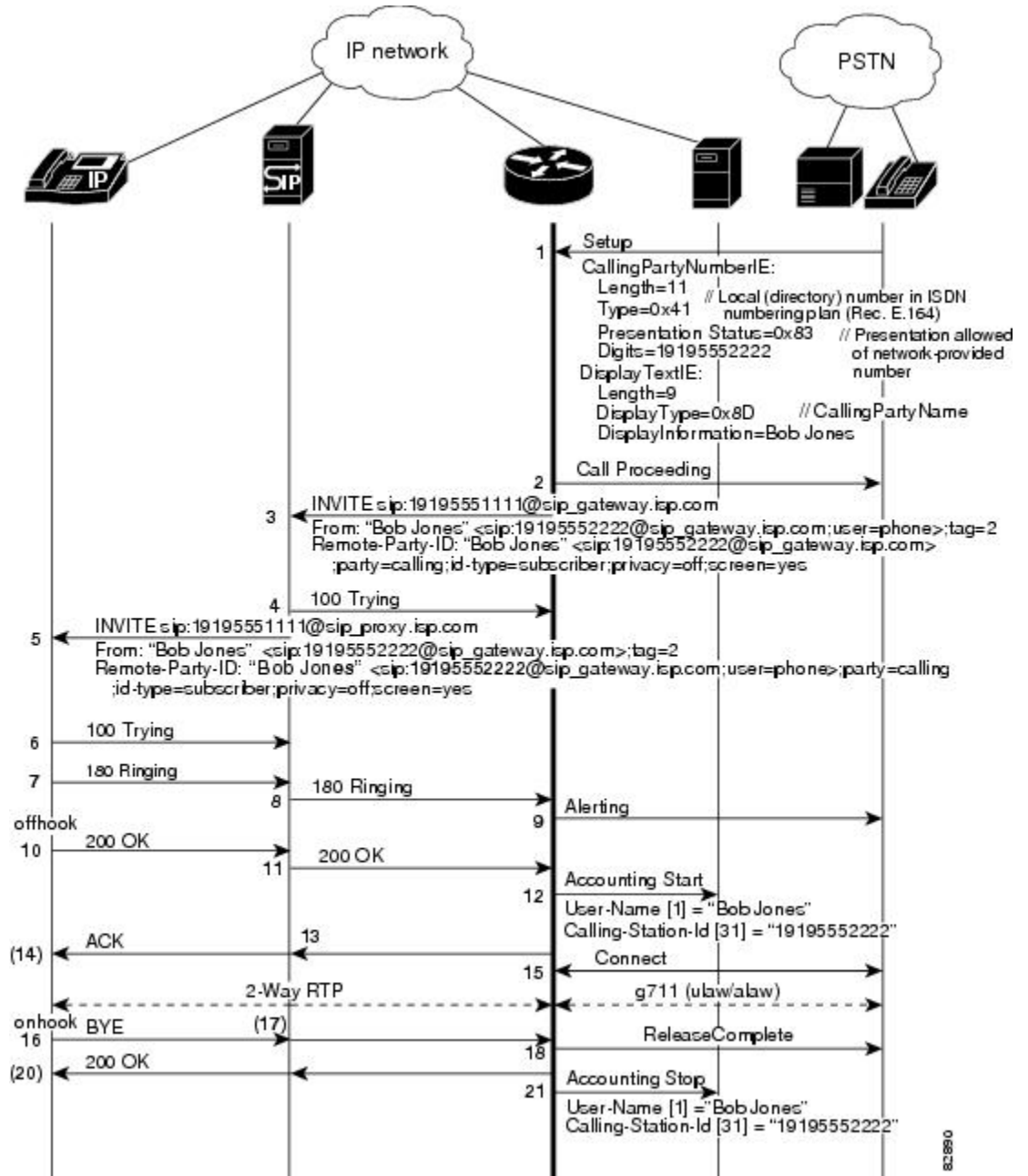
Figure 3: PSTN-to-SIP Default Call Flow with Remote-Party-ID Translation, No Privacy Requested
