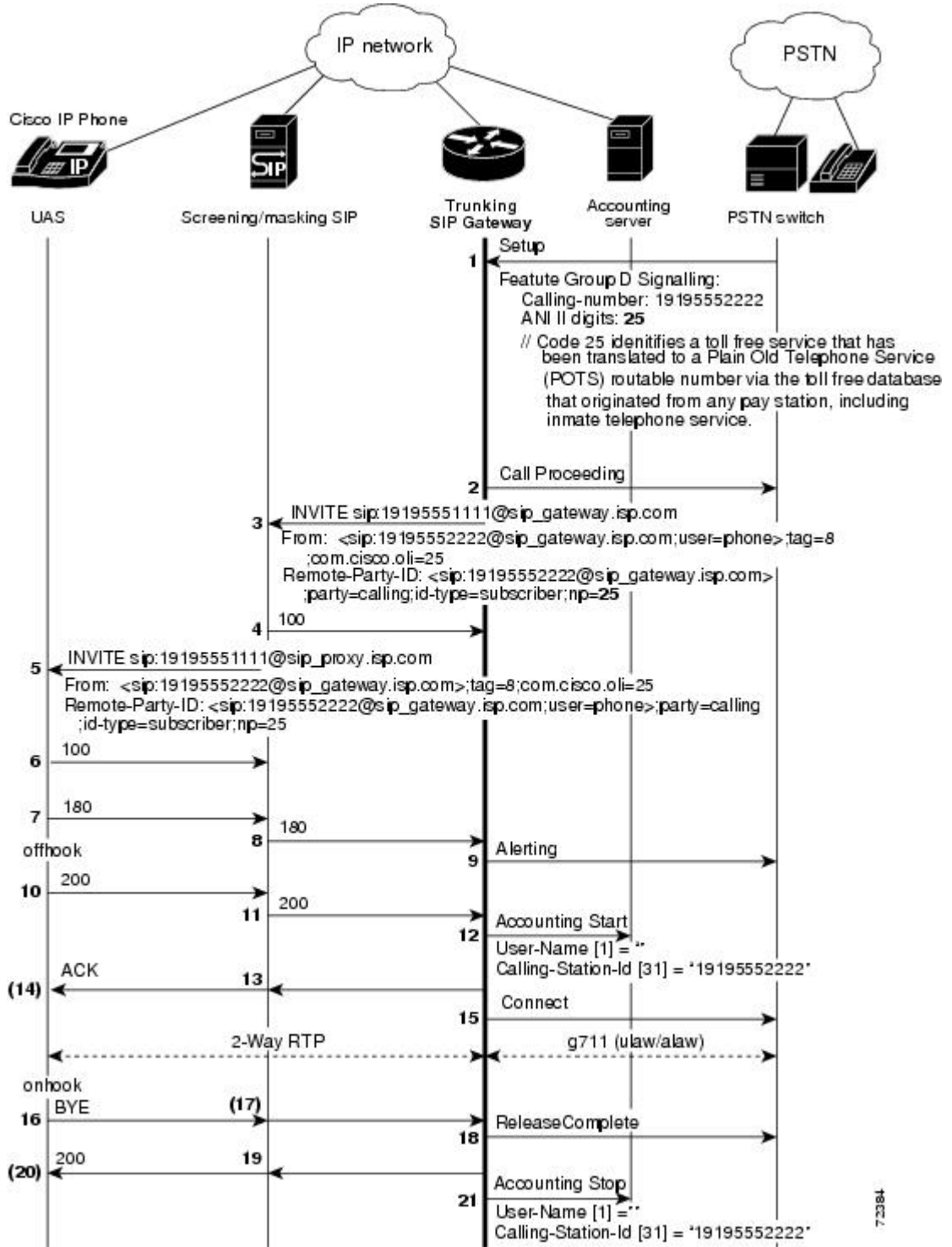
Figure 7: Passing OLI from CAS to SIP
