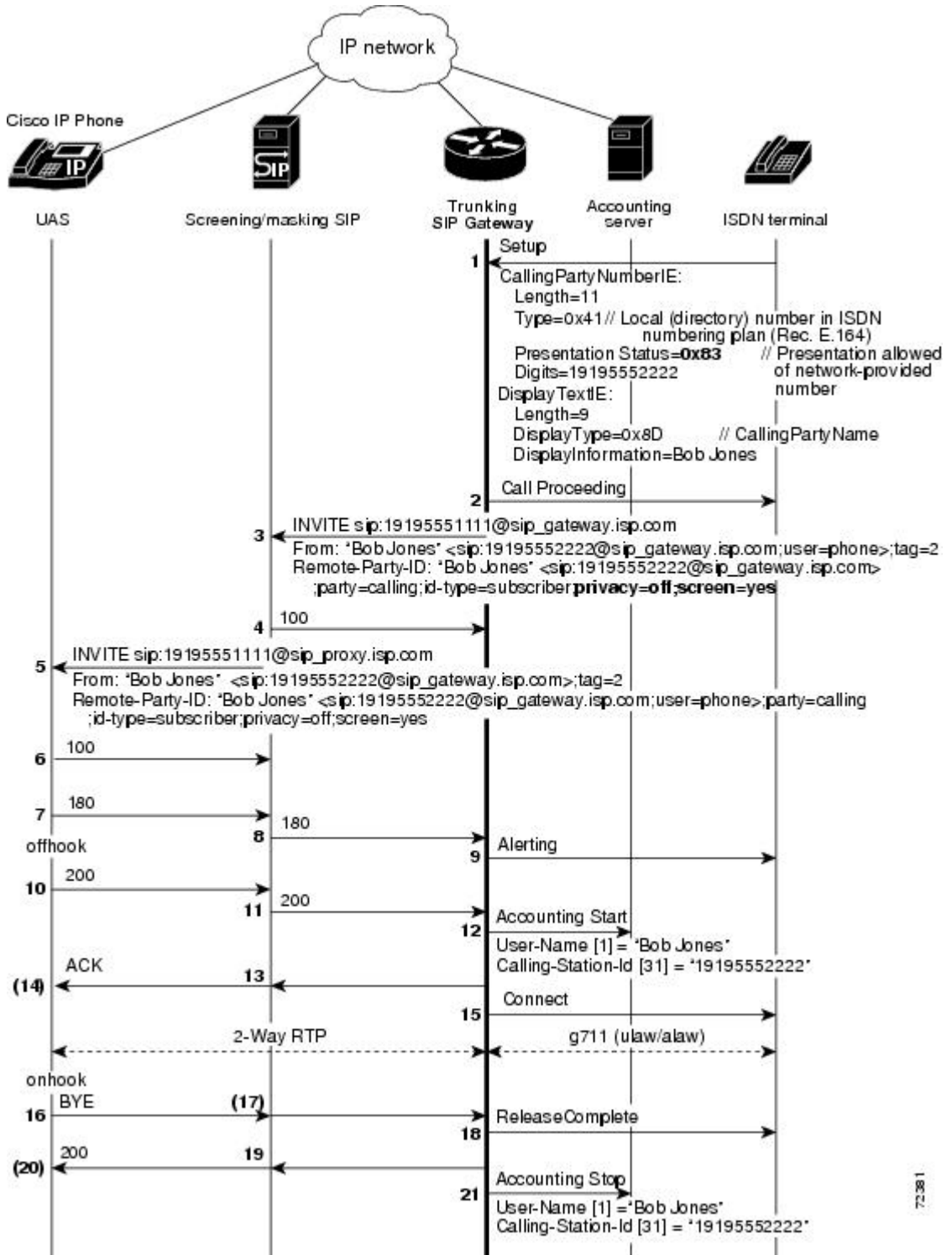
Figure 8: PSTN-to-SIP Call Flow with Remote-Party-ID Translation, No Privacy Requested
