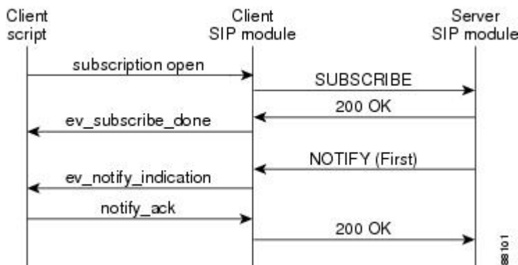
Figure 14: Successful Subscription
