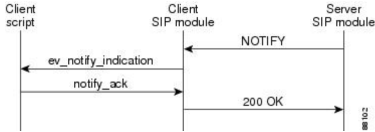
Figure 15: Subscription Completed
