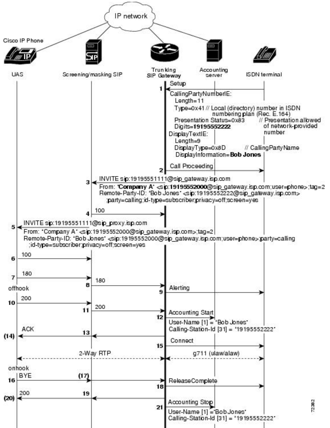
Figure 6: Overriding Calling Name and Number of From Header
