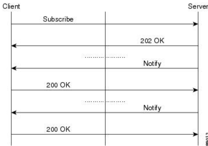
Figure 13: SUBSCRIBE and NOTIFY Message Flow
