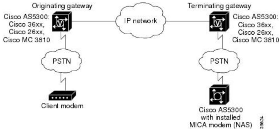
Figure 16: Modem Pass Through Connection Example
