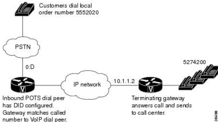
Figure 14: VoIP Call Using DID
