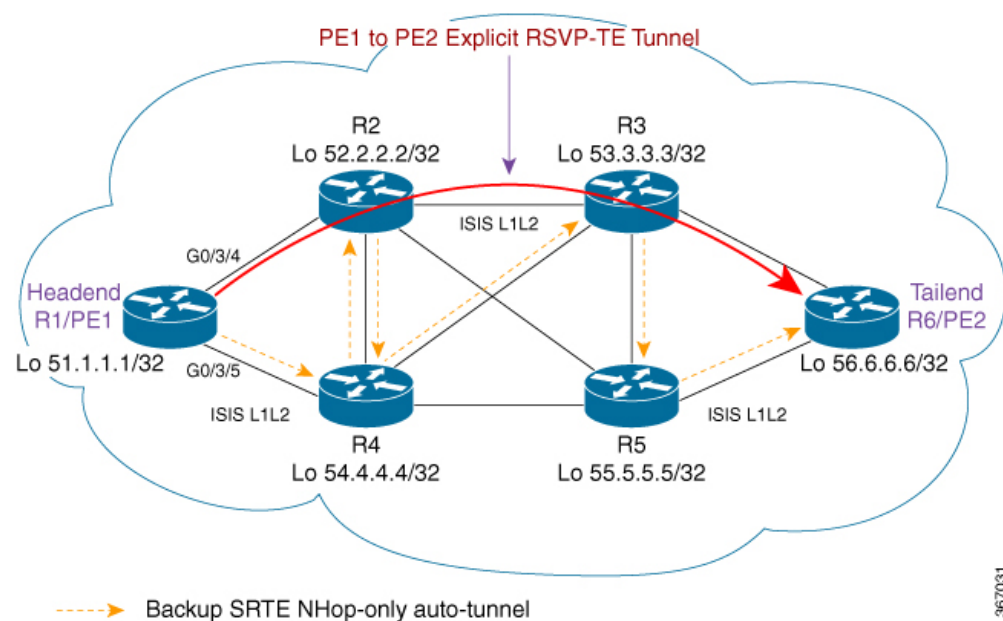
Figure 3: Explicit RSVP-TE Tunnel
