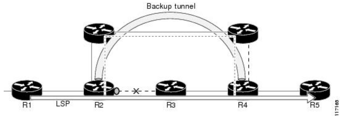
Figure 25: Backup Tunnel in the Same SRLG as the Interface It Is Protecting
