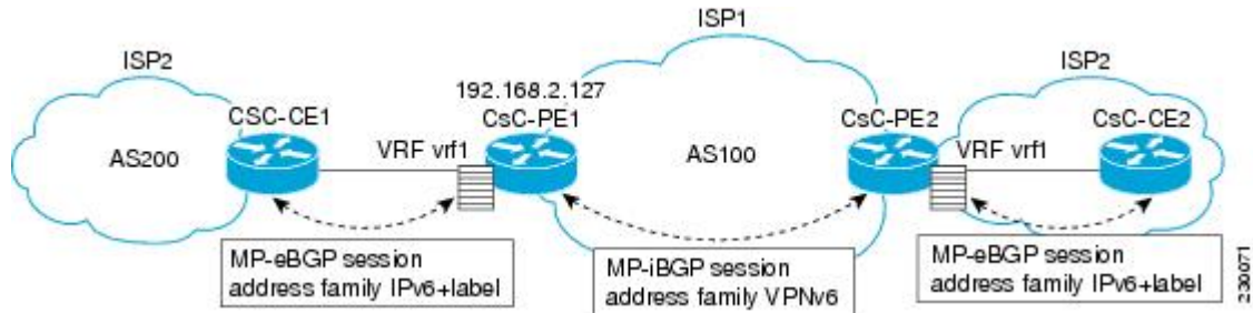
Figure 37 CSC 6VPE Configuration Example
