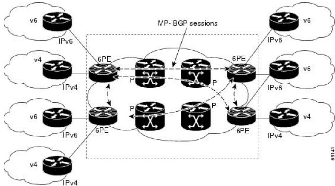
Figure 31 6PE Router Topology
