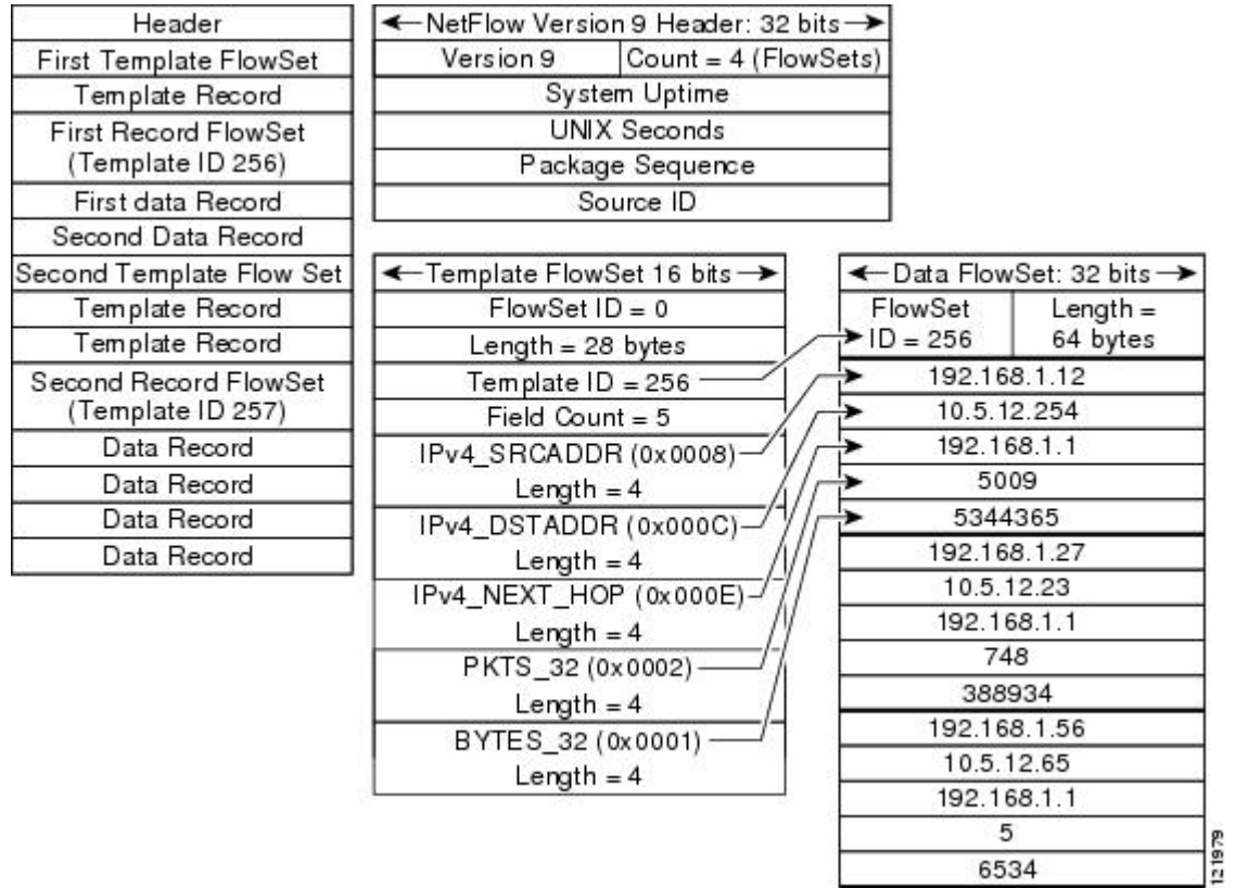
Figure 40 NetFlow Version 9 Export Format Packet Example
