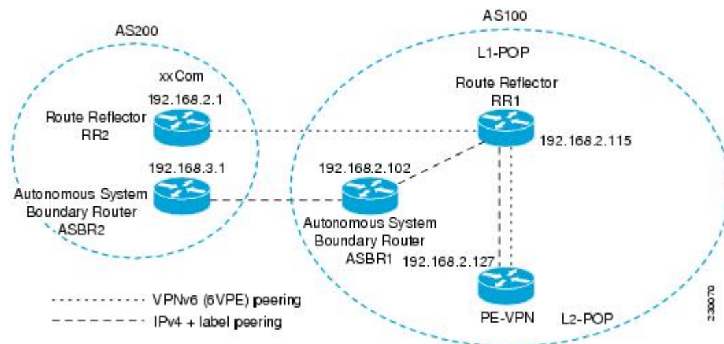
Figure 39 BGP Peering Points for Enabling Interautonomous System Scenario C
