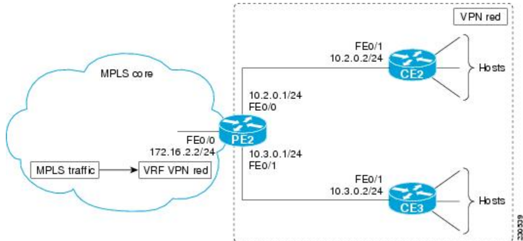
Figure 2: Example of a Router (PE2) Receiving Traffic over a MPLS VPN VRF Interface
