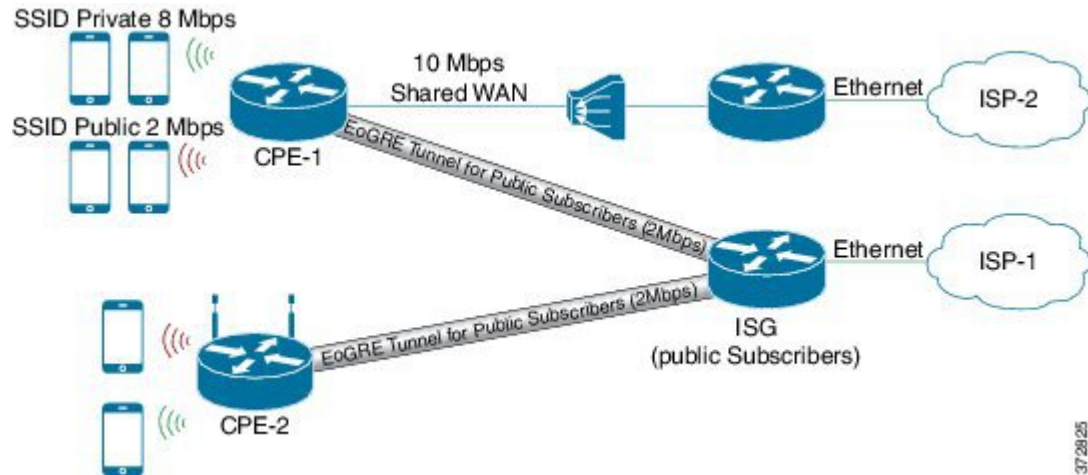
Figure 1: EoGRE Downstream QoS Use Case
