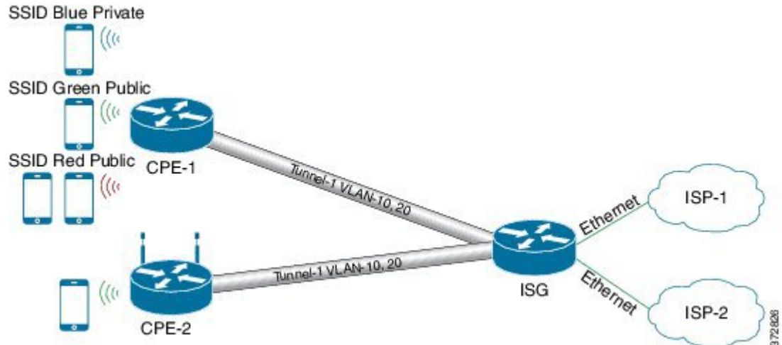
Figure 3: Single Tunnel for Multiple SSIDs
