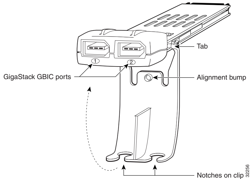
Figure 1 Attaching the GBIC Clip
