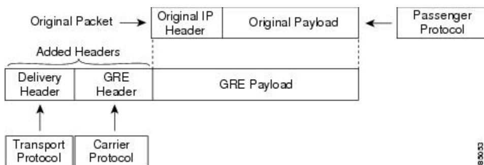
Figure 14: GRE PDU
