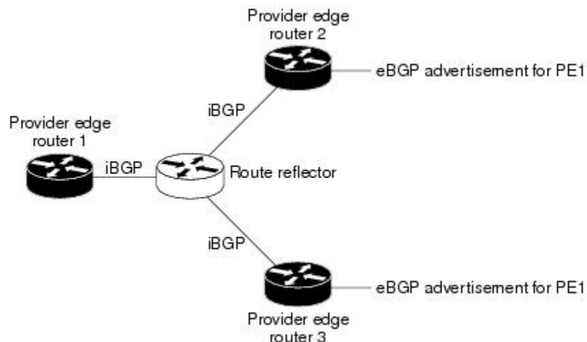
Figure 7: Topology with a Route Reflector
