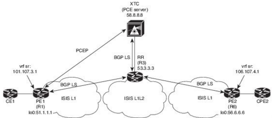
Figure 11: Reference Topology
