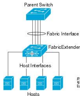
Figure 2: Port Channel Fabric Interface Connection
