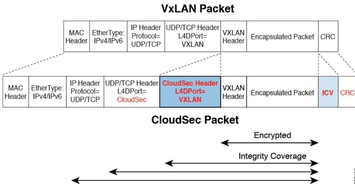
Figure 20: CloudSec Packet
