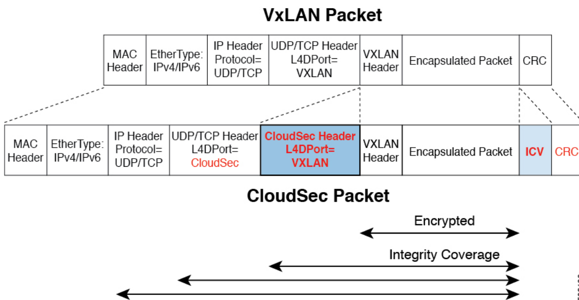
Figure 12: CloudSec Packet
