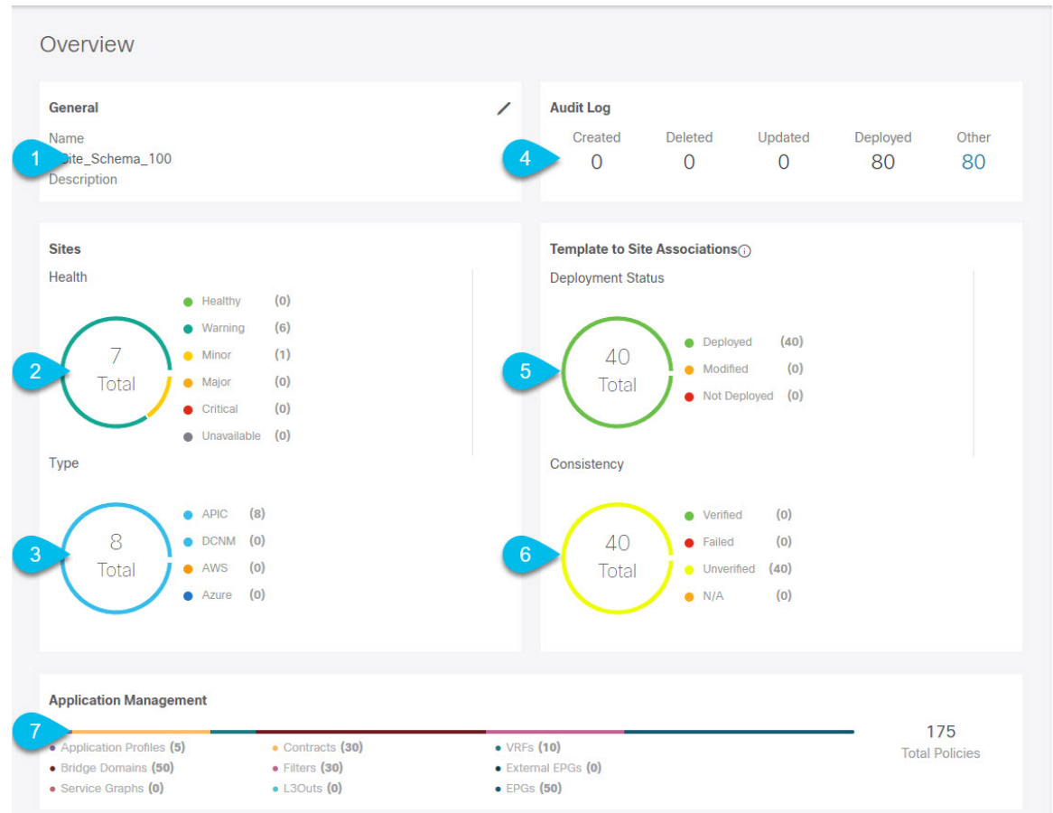
Figure 5: Schema Overview
