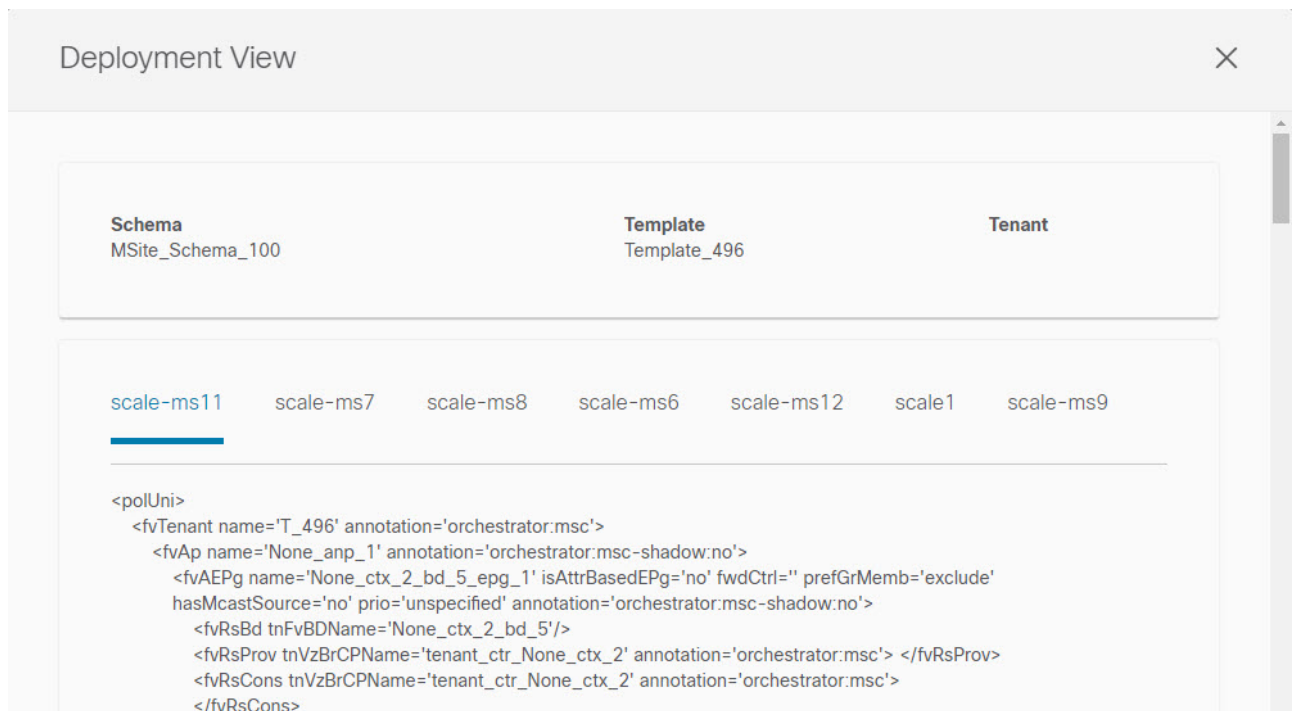
Figure 11. Deployment View
