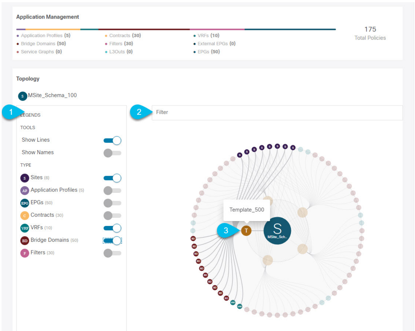
Figure 13. Deployment Visualizer
