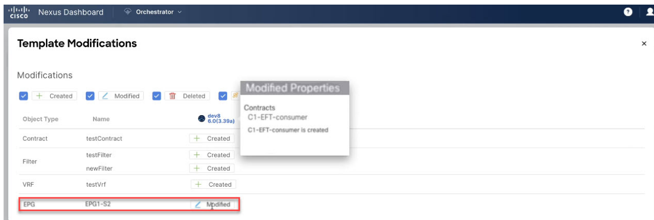
Figure 4. Template Status
