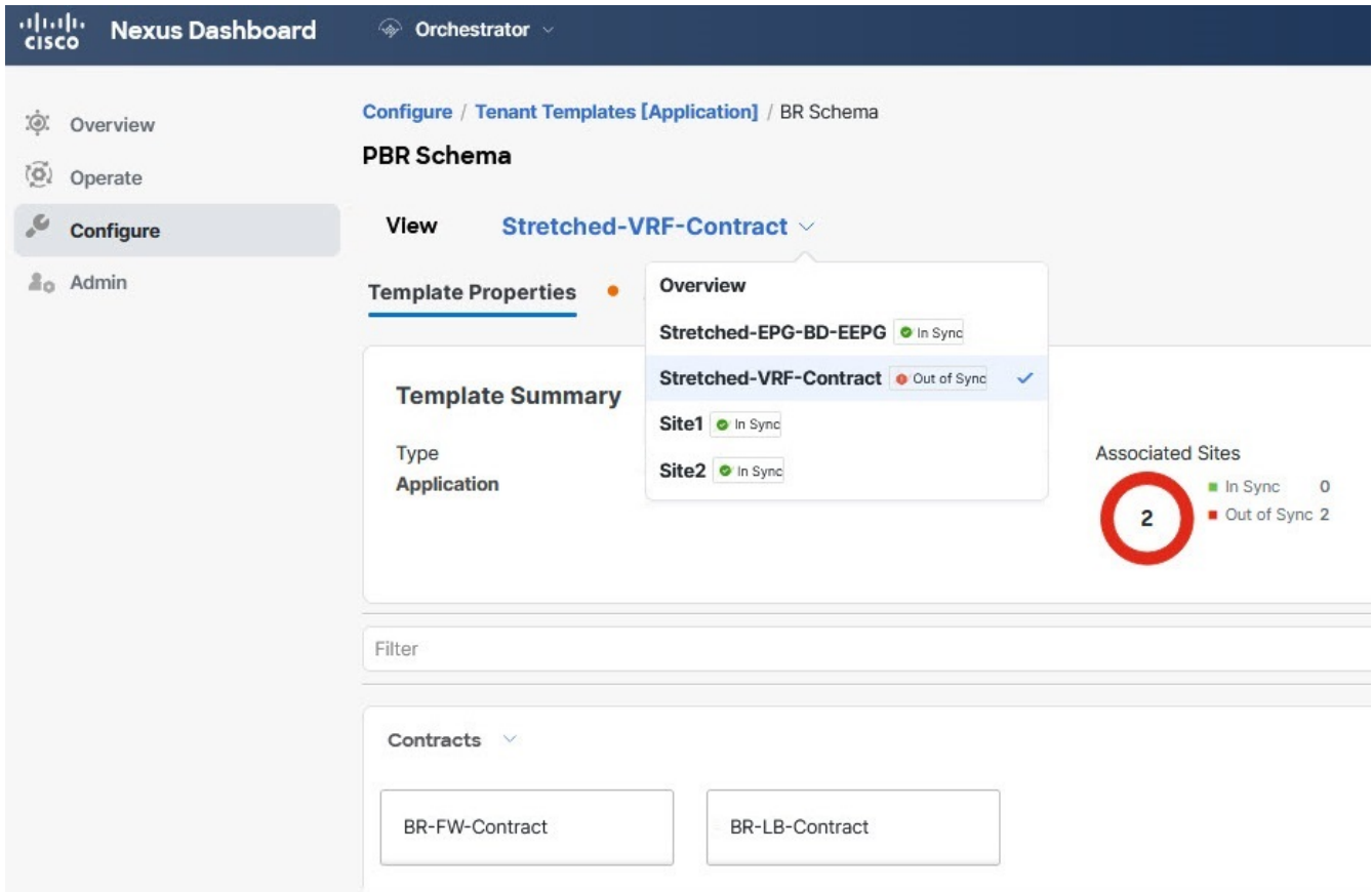
Figure 7. Configuration Drifts
