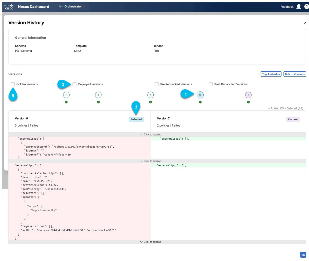
Figure 6. Version History
