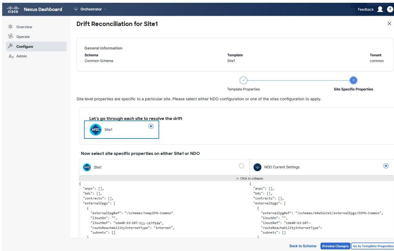
Figure 10. Fabric Specific Properties
