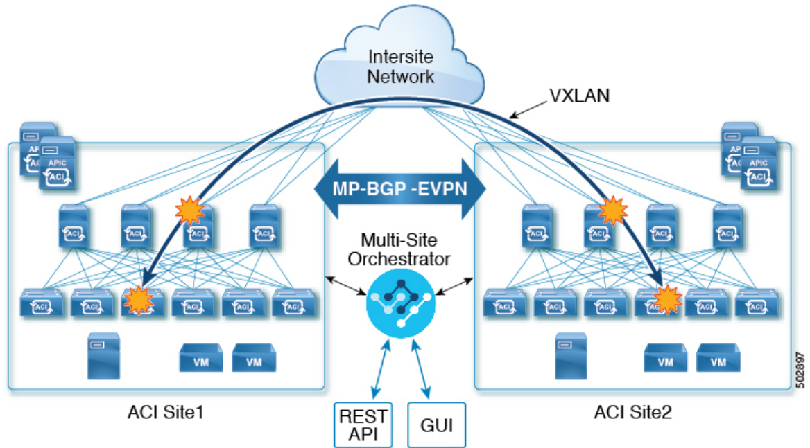
Figure 36: Multi-Site and ISN
