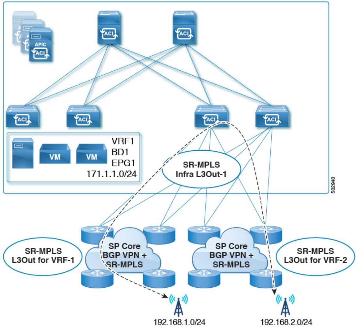
Figure 39: Supported Transit Routing Configuration Using Different VRFs
