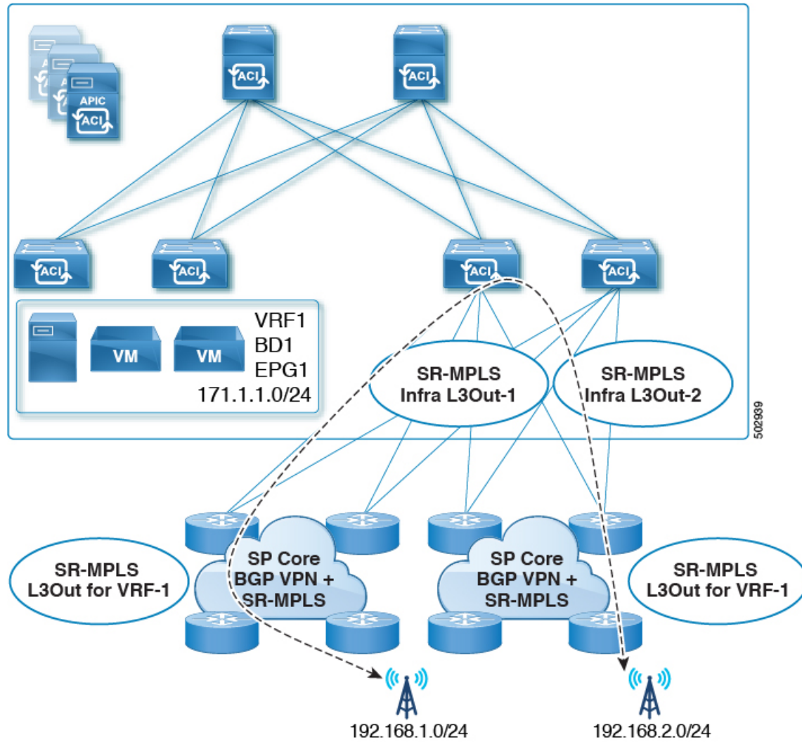
Figure 38: Unsupported Transit Routing Configuration Using Single VRF
