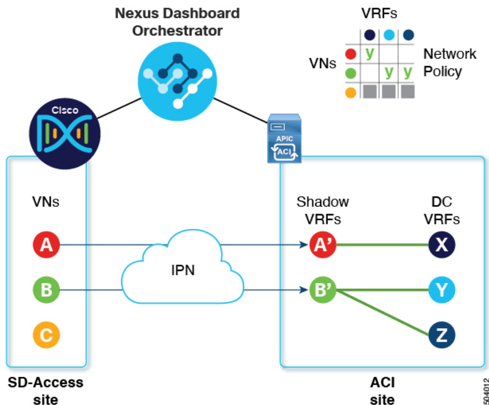
Figure 27: Macro Segmentation using NDO for SD-Access-to-ACI integration
