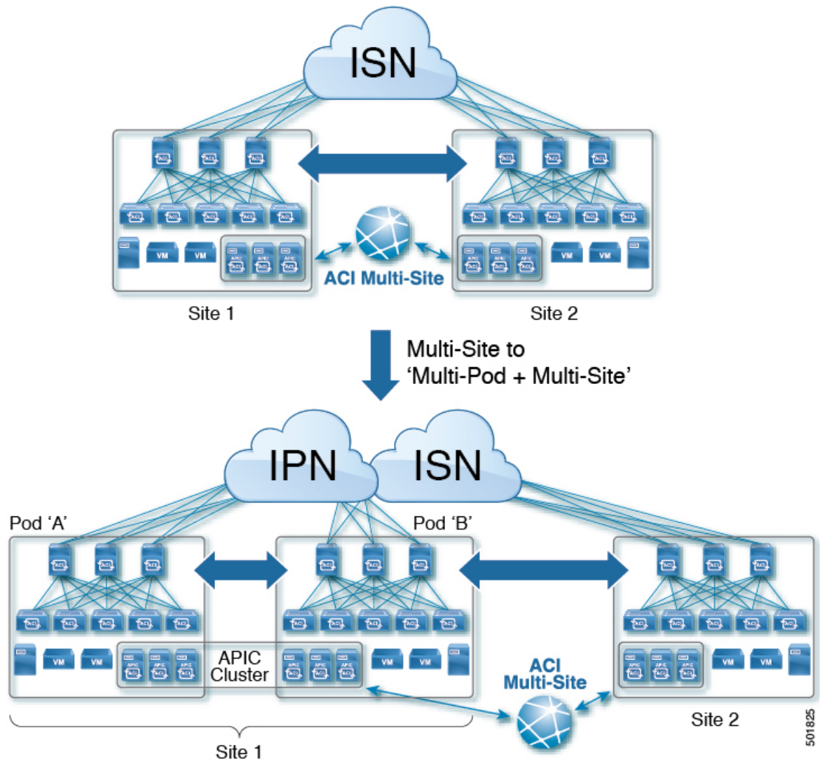
Figure 25: Converting a single POD site in Multi-Site to a multipod site
