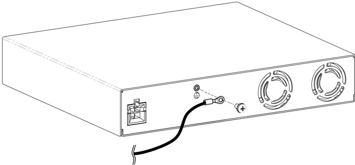
Figure 5: Fasten the Ground Lug
