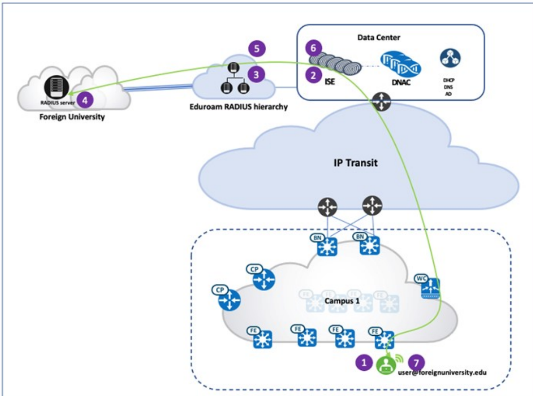
Figure 8: External User Authentication Flow
