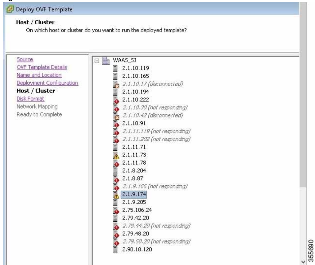
Figure 4-21 Host/Cluster Window
