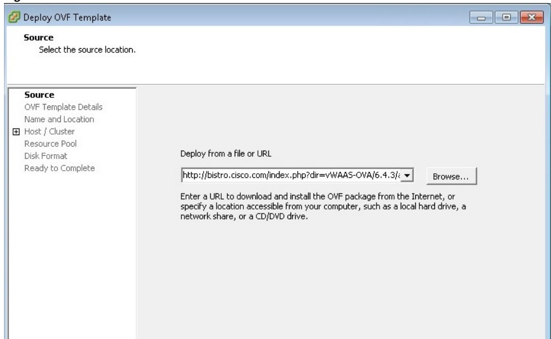
Figure 4-17 Source Window
