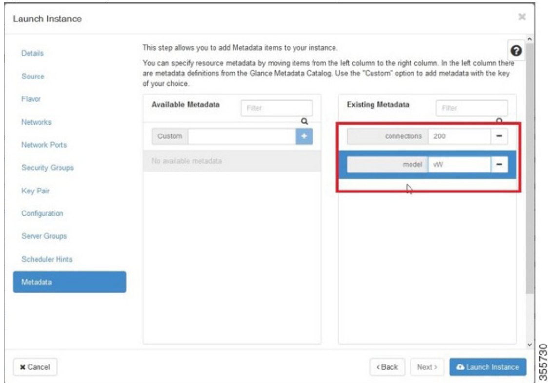
Figure 10-11 OpenStack Launch Instance &gt; Metadata Page
