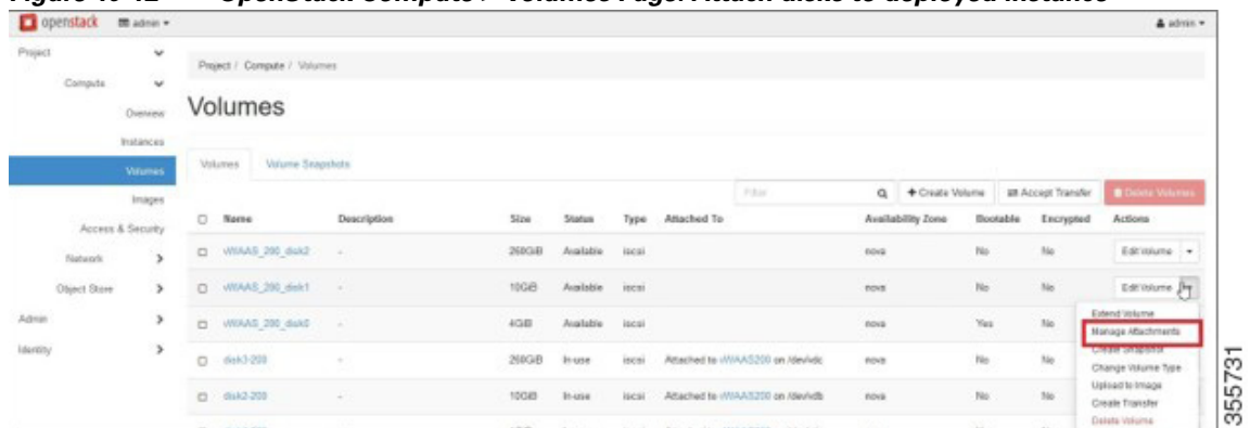
Figure 10-12 OpenStack Compute &gt; Volumes Page: Attach disks to deployed instance
