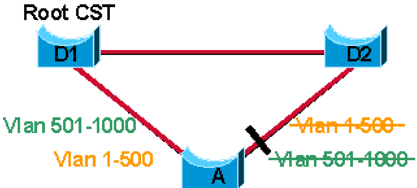
Common Spanning Tree (CST) Applied to Network
