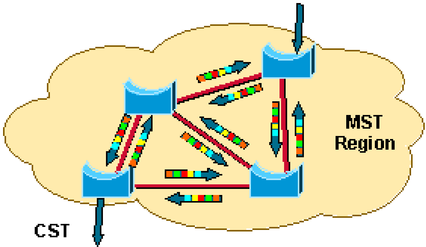
MST BDPUs Sent Inside and Outside of an MST Region
