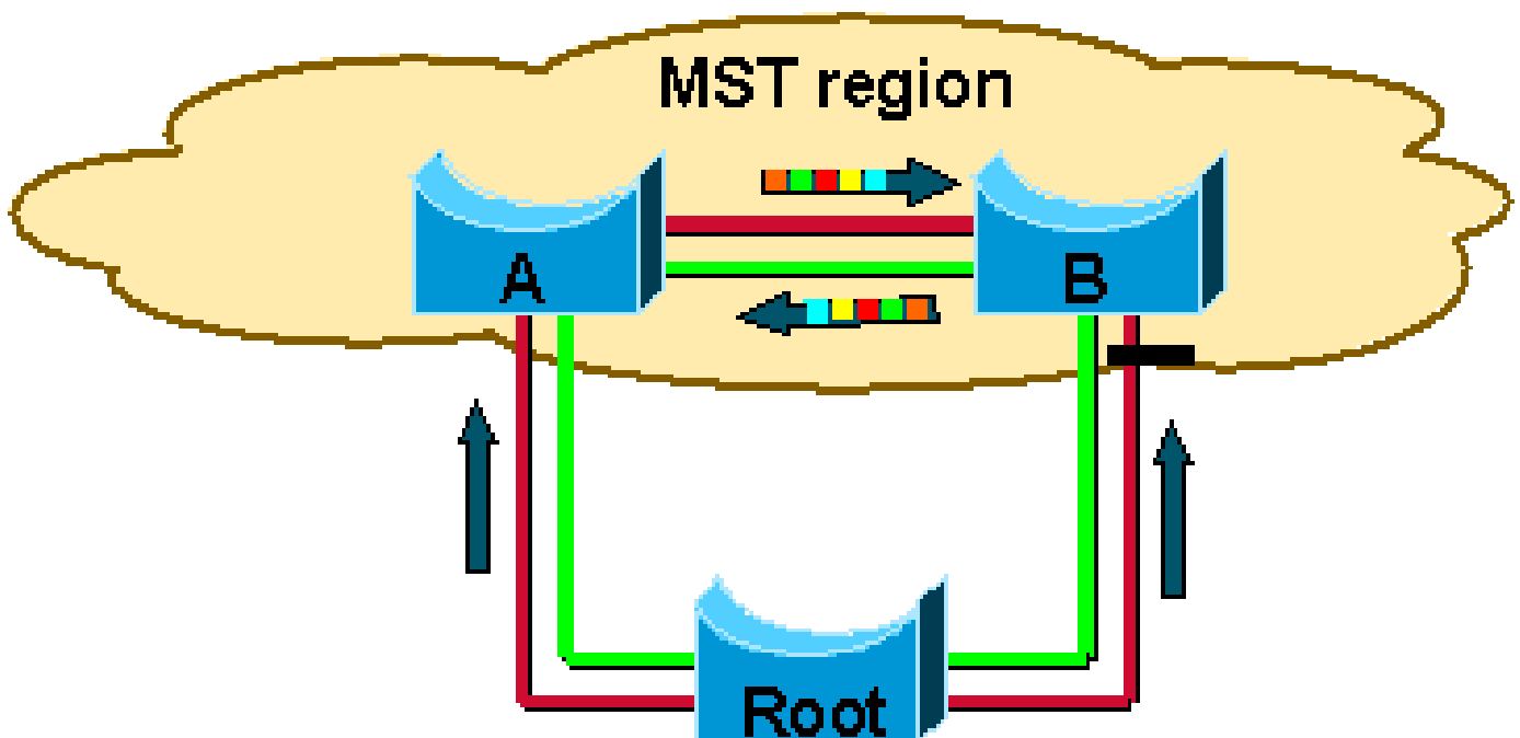
Internal Instances (MSTIs) Always Automatically Match the IST Topology at Boundary Ports
